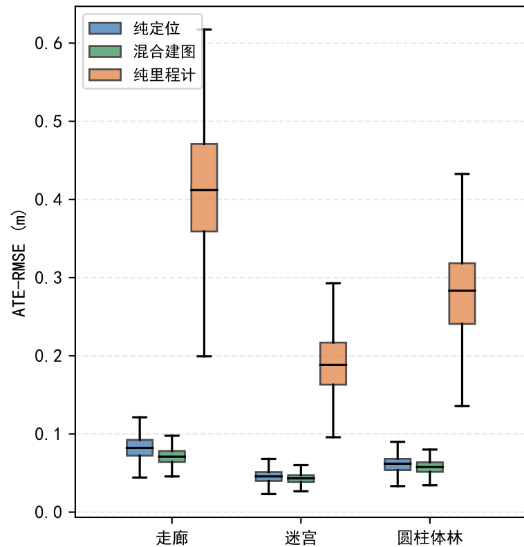
ATE 箱线图对比
