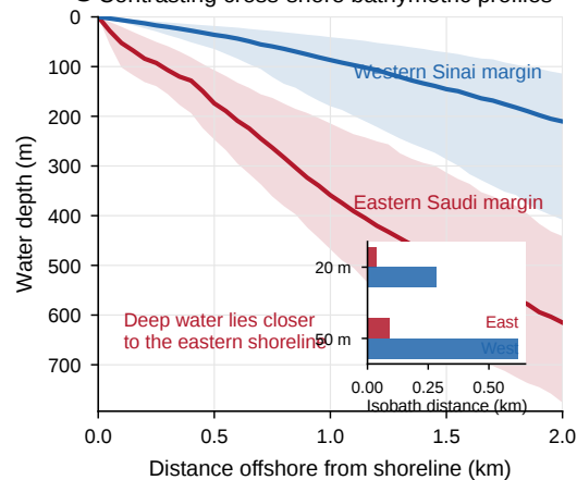
C Contrasting cross-shore bathymetric profiles
