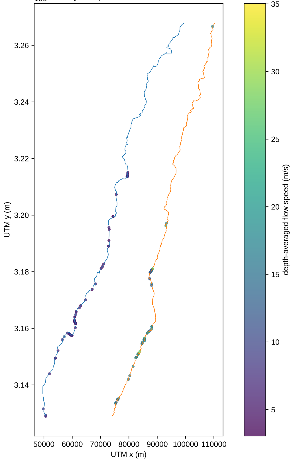
1e6 velocity hotspots over shoreline stations
