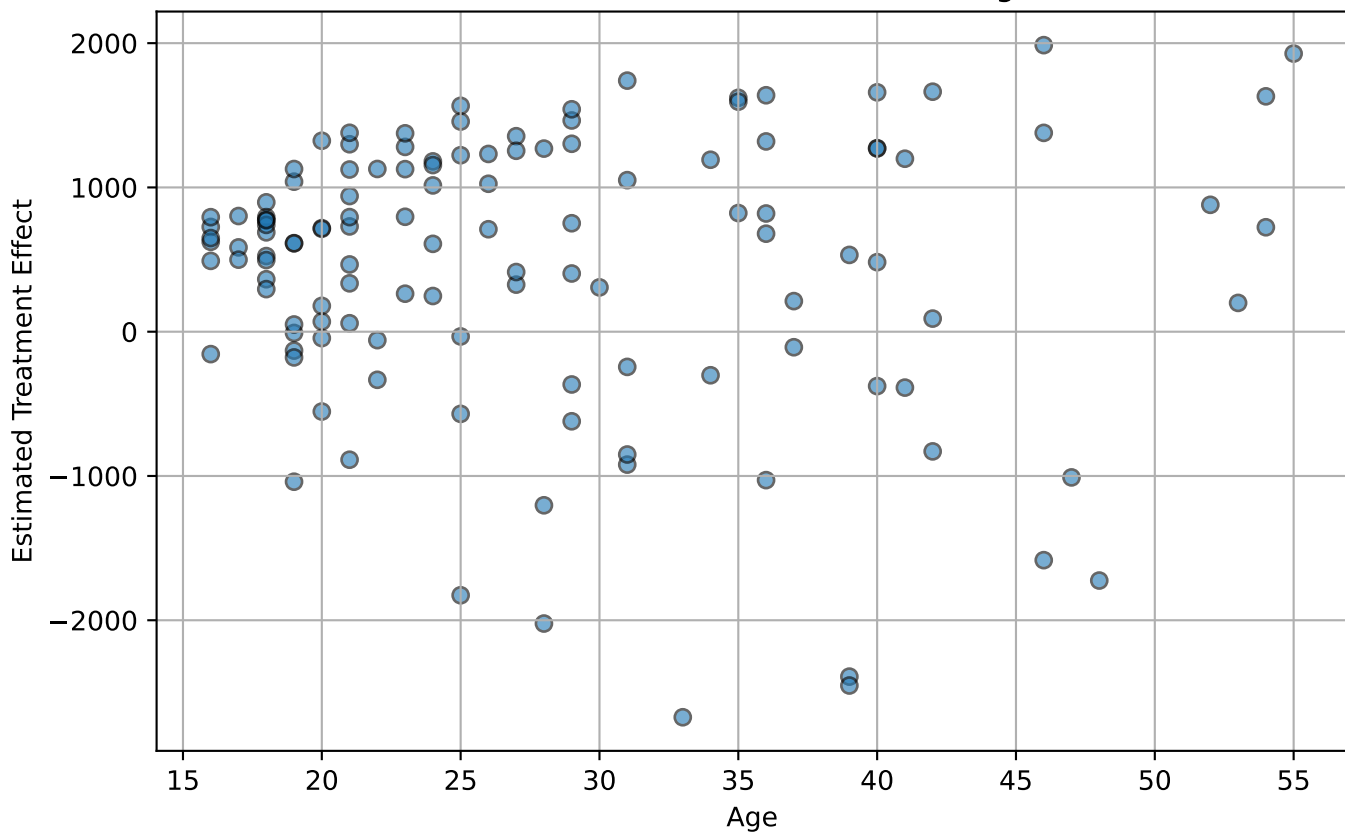
Estimated Treatment Effect vs. Age
