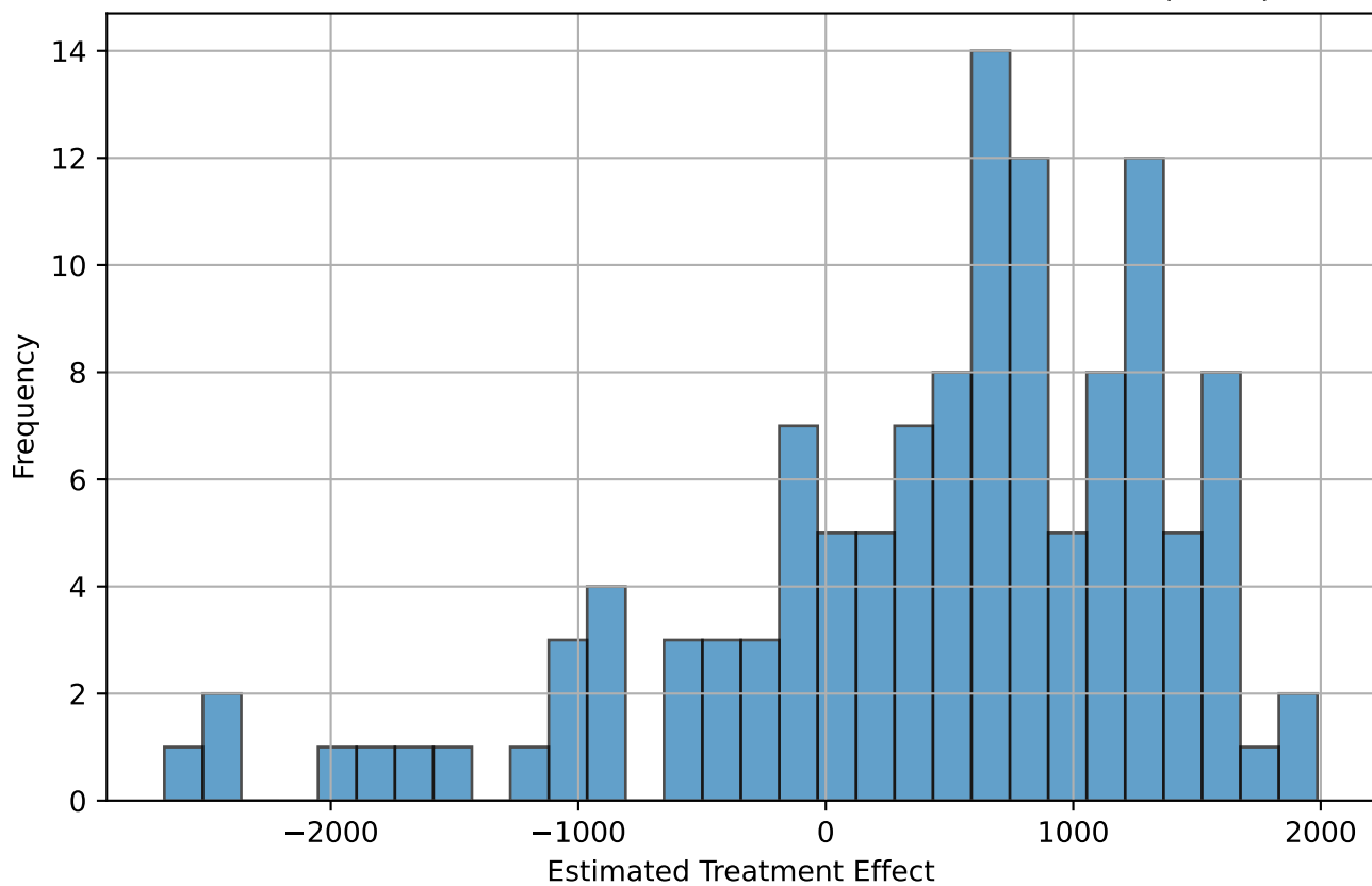
Distribution of Estimated Conditional Treatment Effects (CATE)
