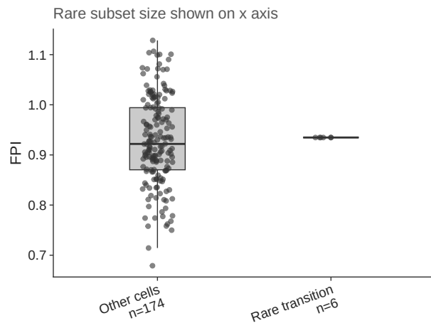
D FPI in simulator-labeled transition cells
