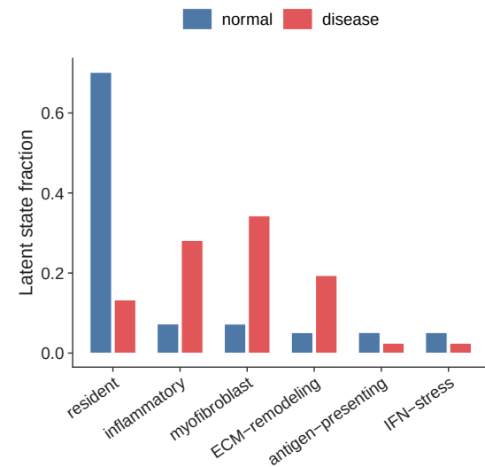
C Fibroblast Plasticity Index by condition
