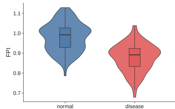
C Fibroblast Plasticity Index by condition
