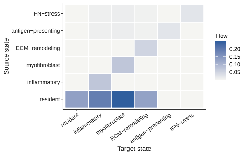
D FPI in simulator-labeled transition cells
