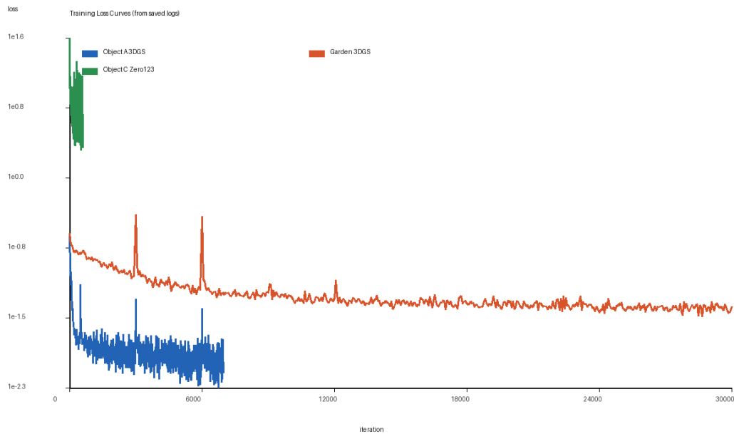
Figure 2: Training curves parsed from saved logs. The console log for Object B does not contain scalar loss values; the complete scalar records are available in the W&B run.
