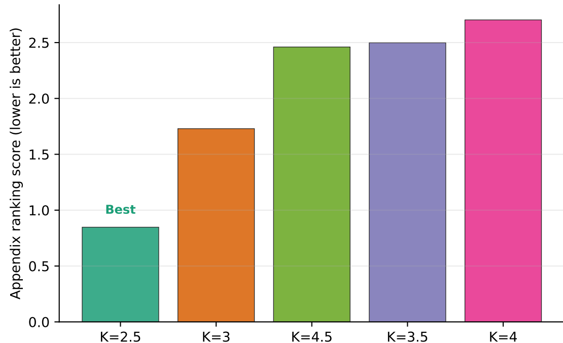
Kuramoto K ranking (appendix sweep)
