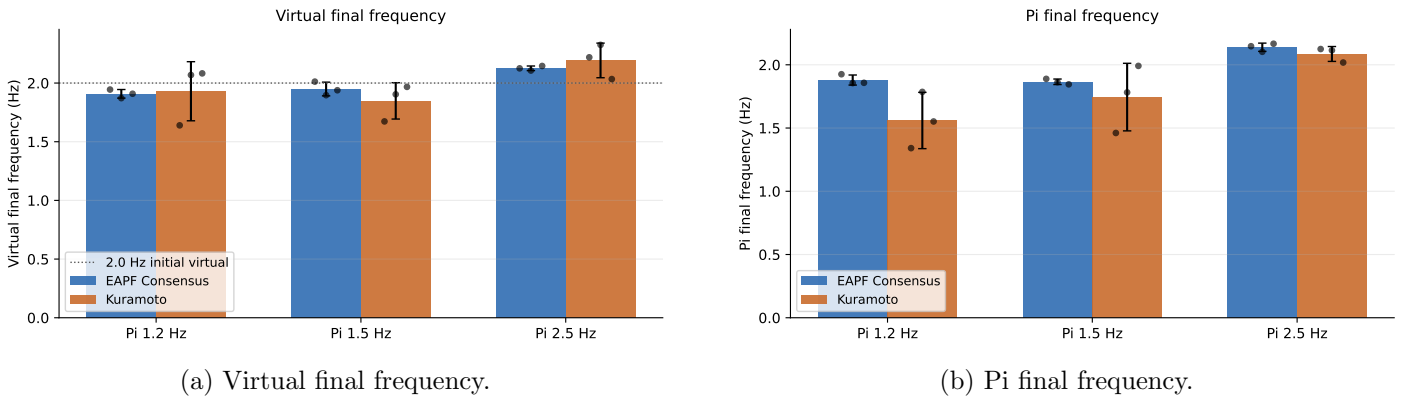
Figure 2: Final 5 s mean frequencies by model and condition. Bars show model-condition means and black points show individual trials. The dashed line marks the nominal initial virtual frequency of 2.0 Hz; in the bidirectional mutual HIL loop this is not treated as a fixed reference target, since both agents can adapt.
