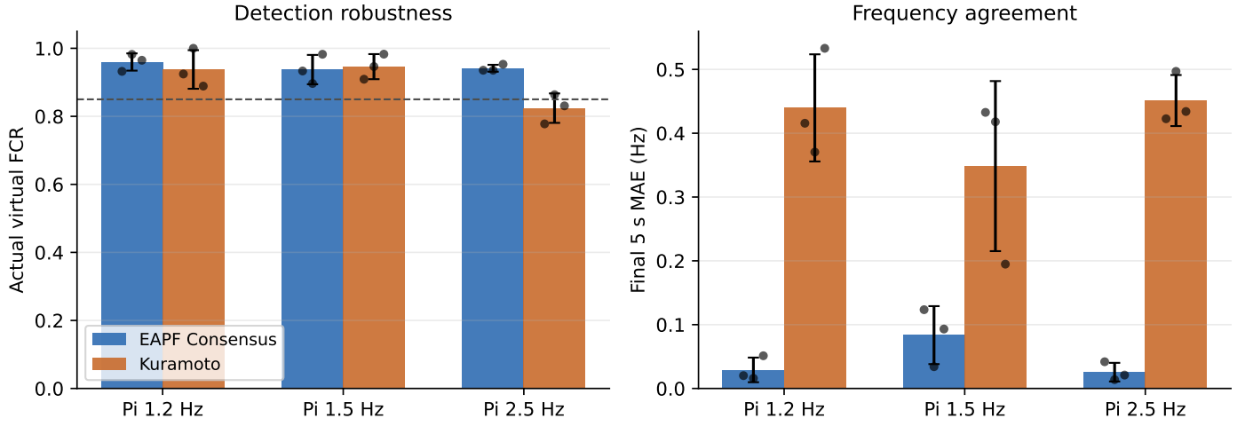
Figure 1: Mutual HIL robustness overview (1 virtual + 1 Pi, 30 s trials). Bars show mean across three repeats per model-condition pair; black points show individual trial values. The dashed line in the left panel marks an indicative actual-FCR threshold of 0.85.
