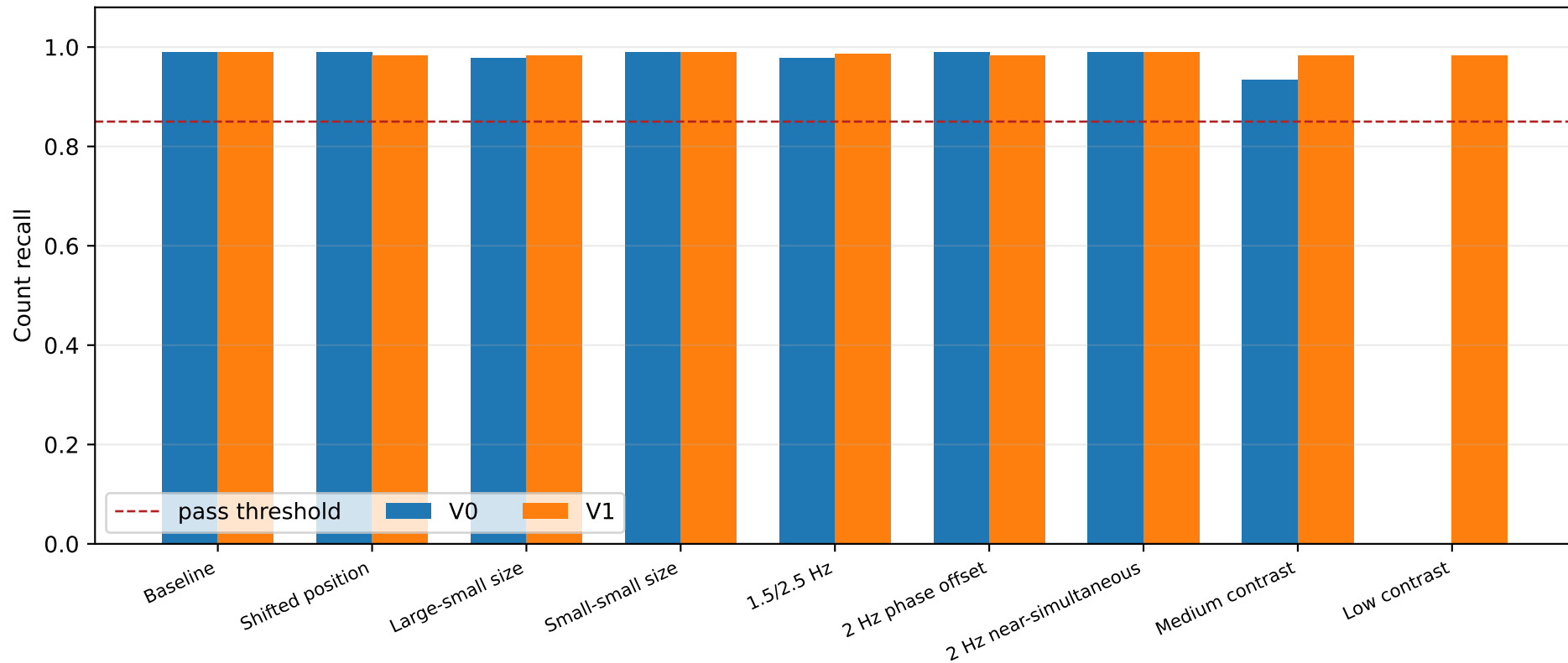
Detection count recall by required condition
