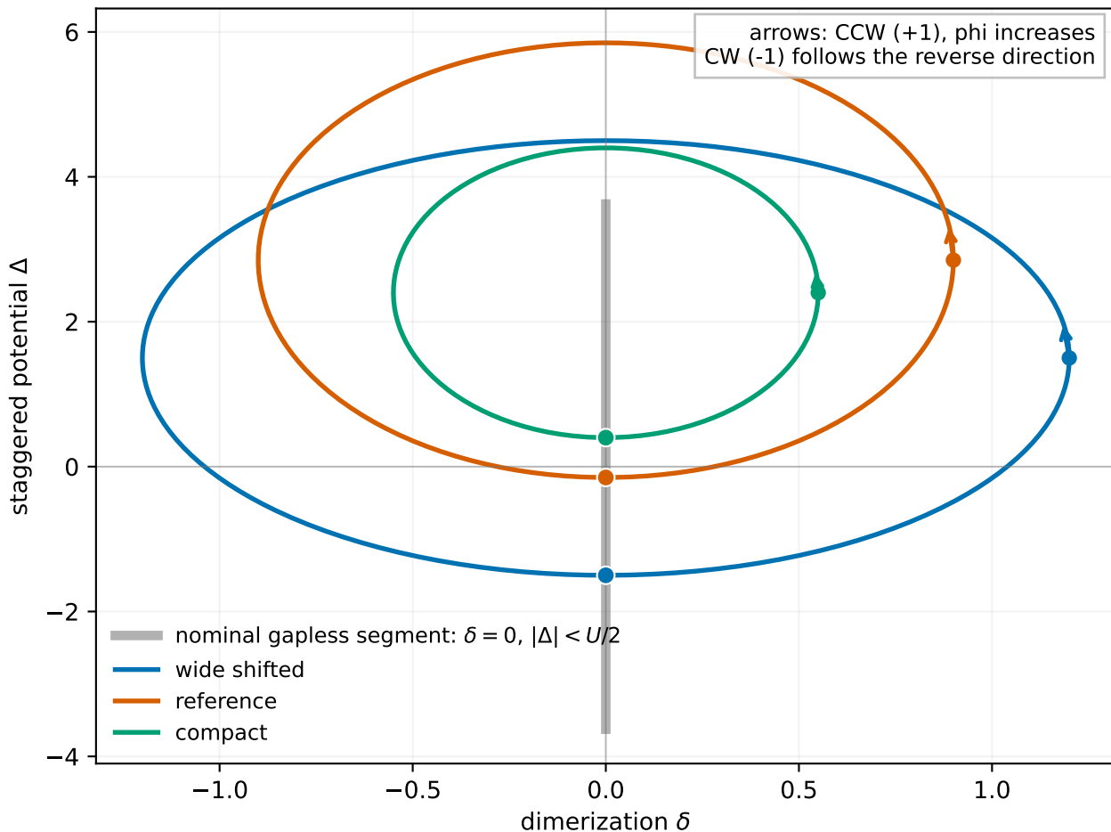
Compared loops at U = 7.25 ; one gapless-line crossing per cycle
