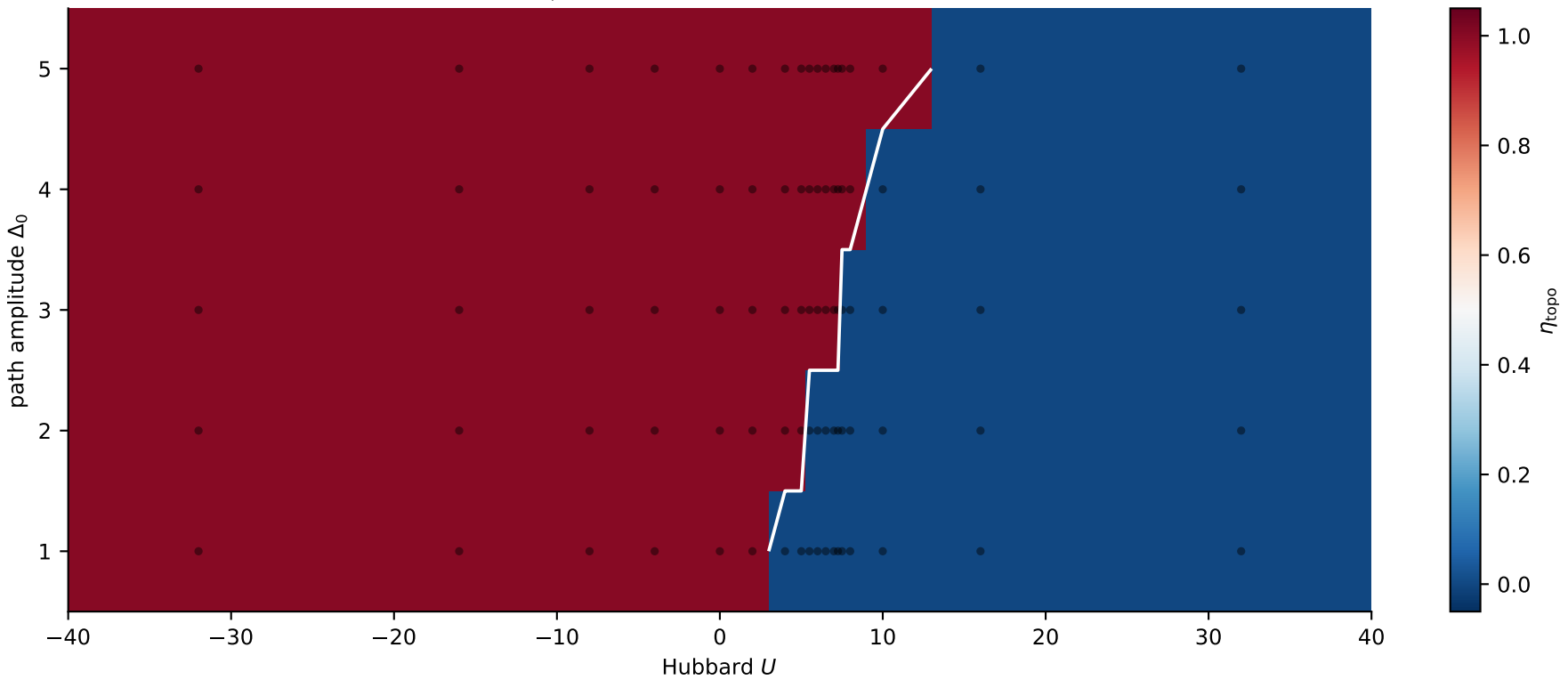
Twist-averaged topological efficiency \eta_{\text{topo}} = C_{\text{MB}}/2
