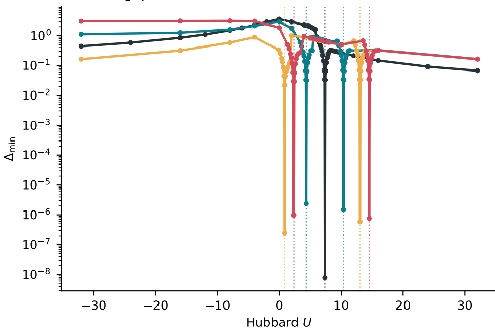
(c) Torus gap with critical-line refinement
