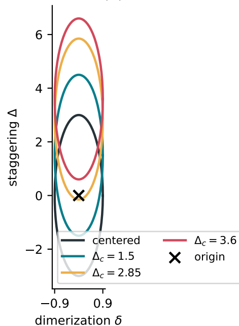
(c) Torus gap with critical-line refinement
