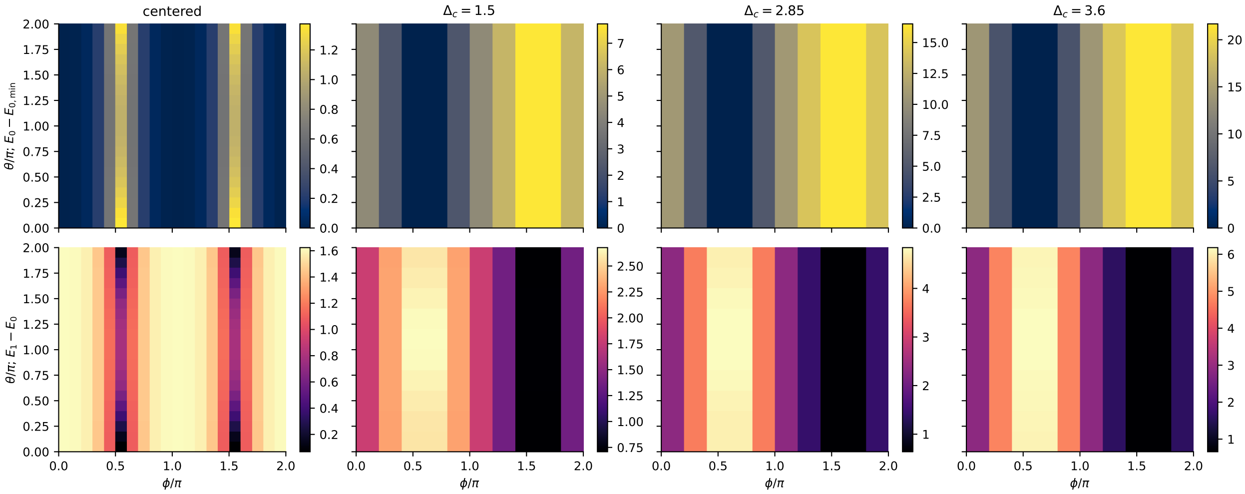
Path-resolved torus spectrum at L = 8, t = 1, U = 7.25
