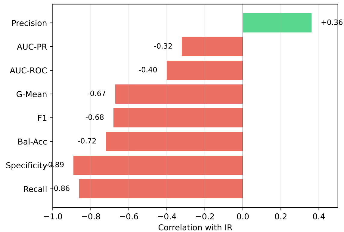
(C) Multi-Metric Validation 8 Evaluation Metrics
