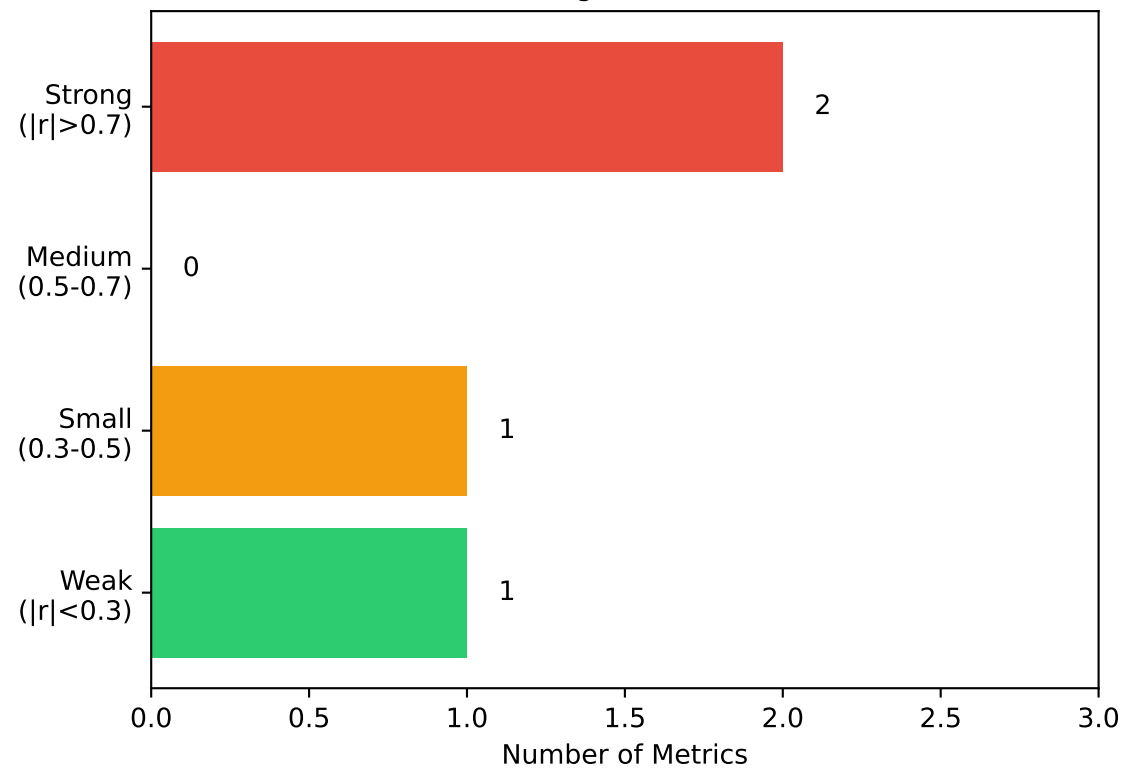
(B) Effect Size Distribution (Ceiling-Controlled)
