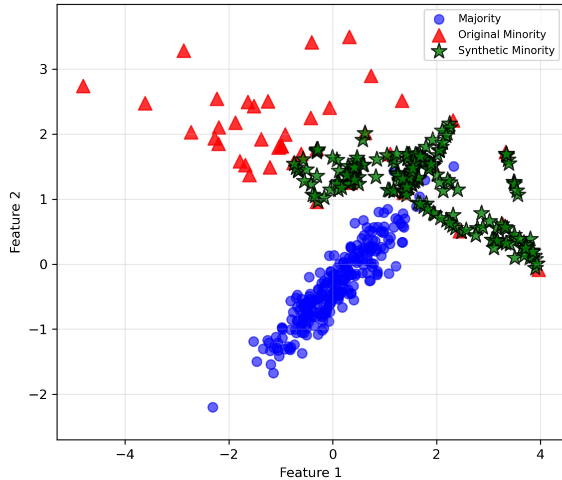
BorderlineSMOTE IR=2.0, n=510
