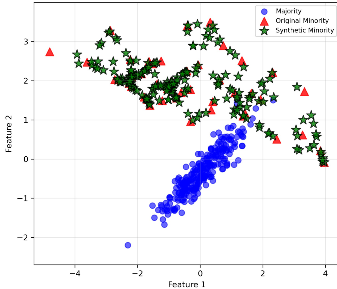
SMOTE IR=2.0, n=510
