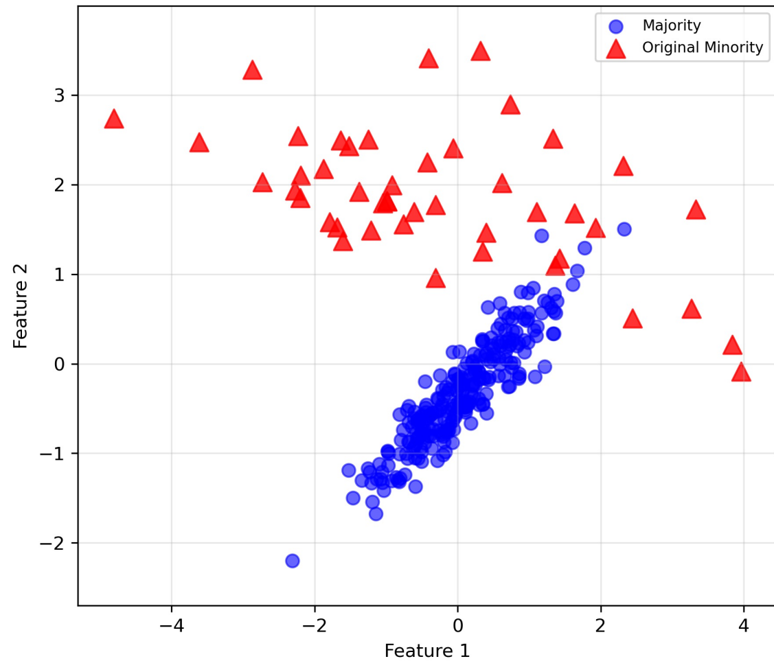
Original IR=6.7, n=300
