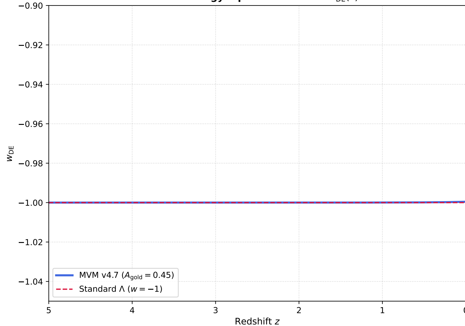
Dark Energy Equation of State w_{DE}(z)
