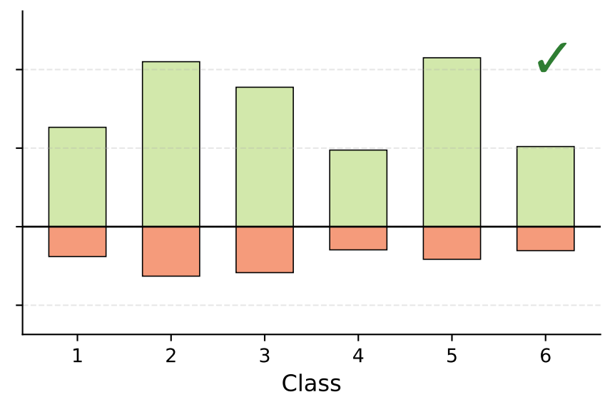
Client 3
