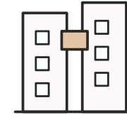
Client 3
