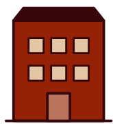
Client 1
