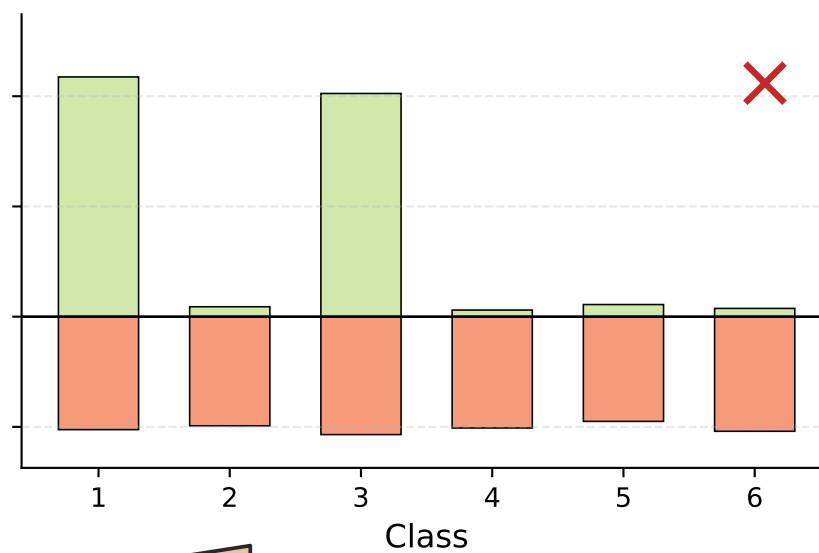
Client 5
