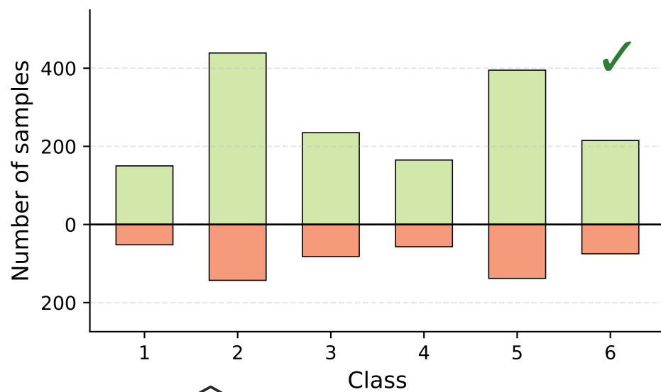
Client 4
