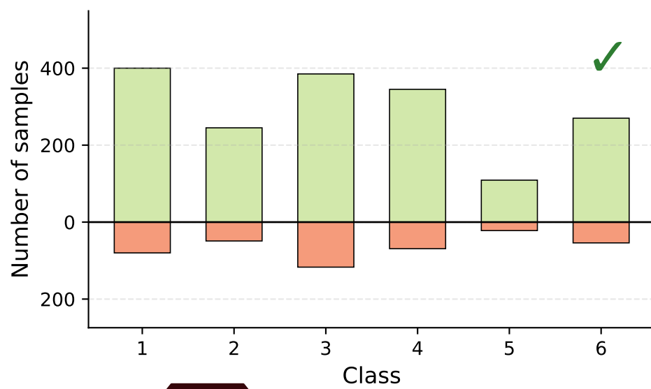
Client 1
