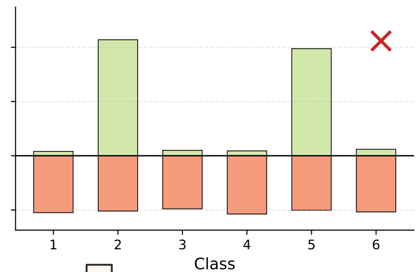
Client 6
