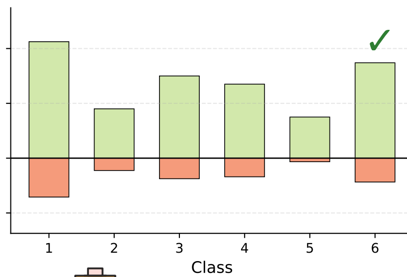
Client 2
