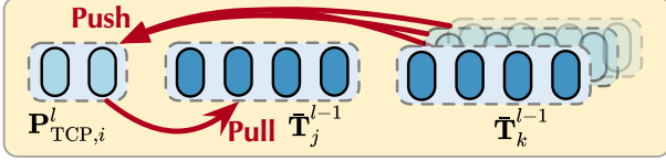
Figure 3. The intra-modal latent consistency regularization.
