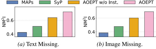
Figure 8. NM²I comparison of AOEPT and baselines on the MM-IMDb dataset with 70% text- or image-missing cases.
