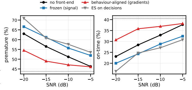
Fig. 2. Freeze-Omni, four systems on 1,000 paired samples per SNR. The signal-trained suppressor makes the eager model take over earlier at every SNR; the behaviour-aligned front-end, same parameters, makes it later, and its gain grows with the acoustic share. Dotted: clean audio.
