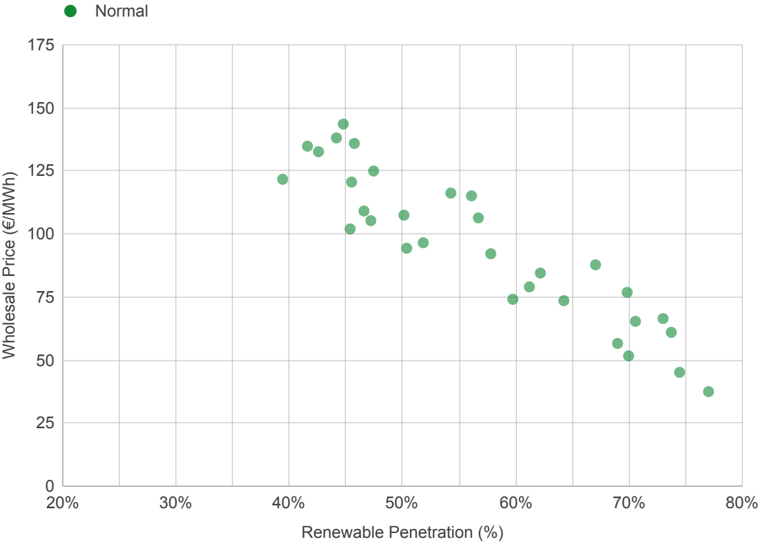
The Merit Order Effect: Renewable Impact on Price
