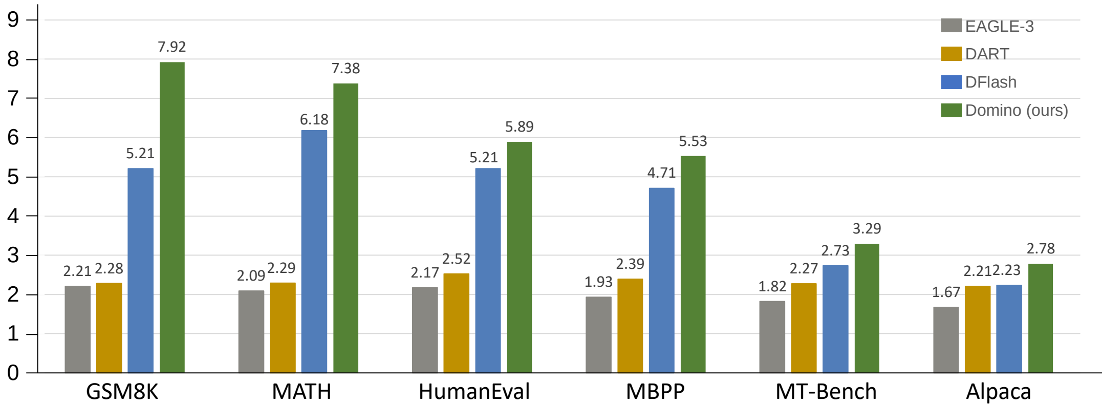
Speedup(x)
