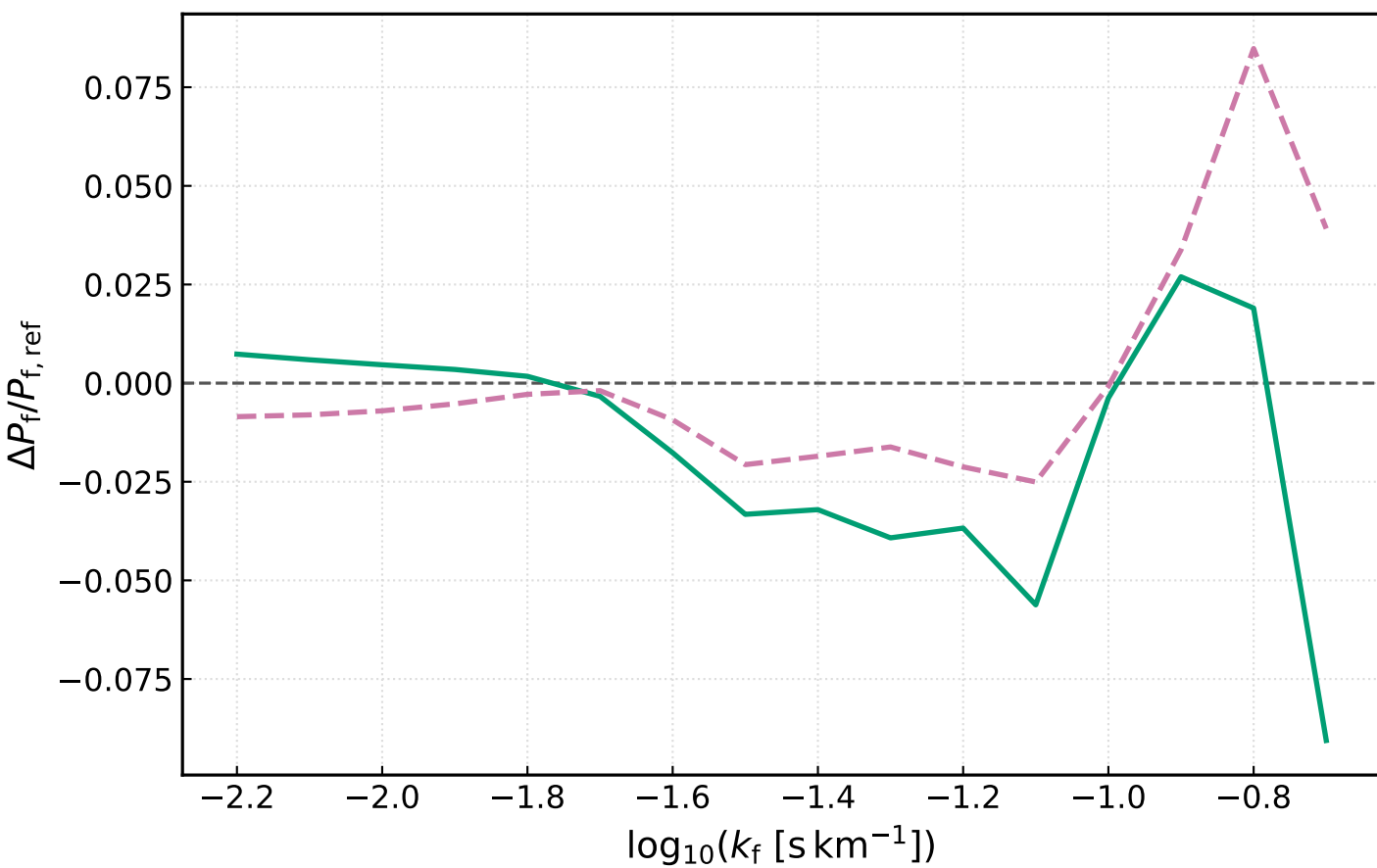
z = 4.2 : Mass Resolution Relative Diff
