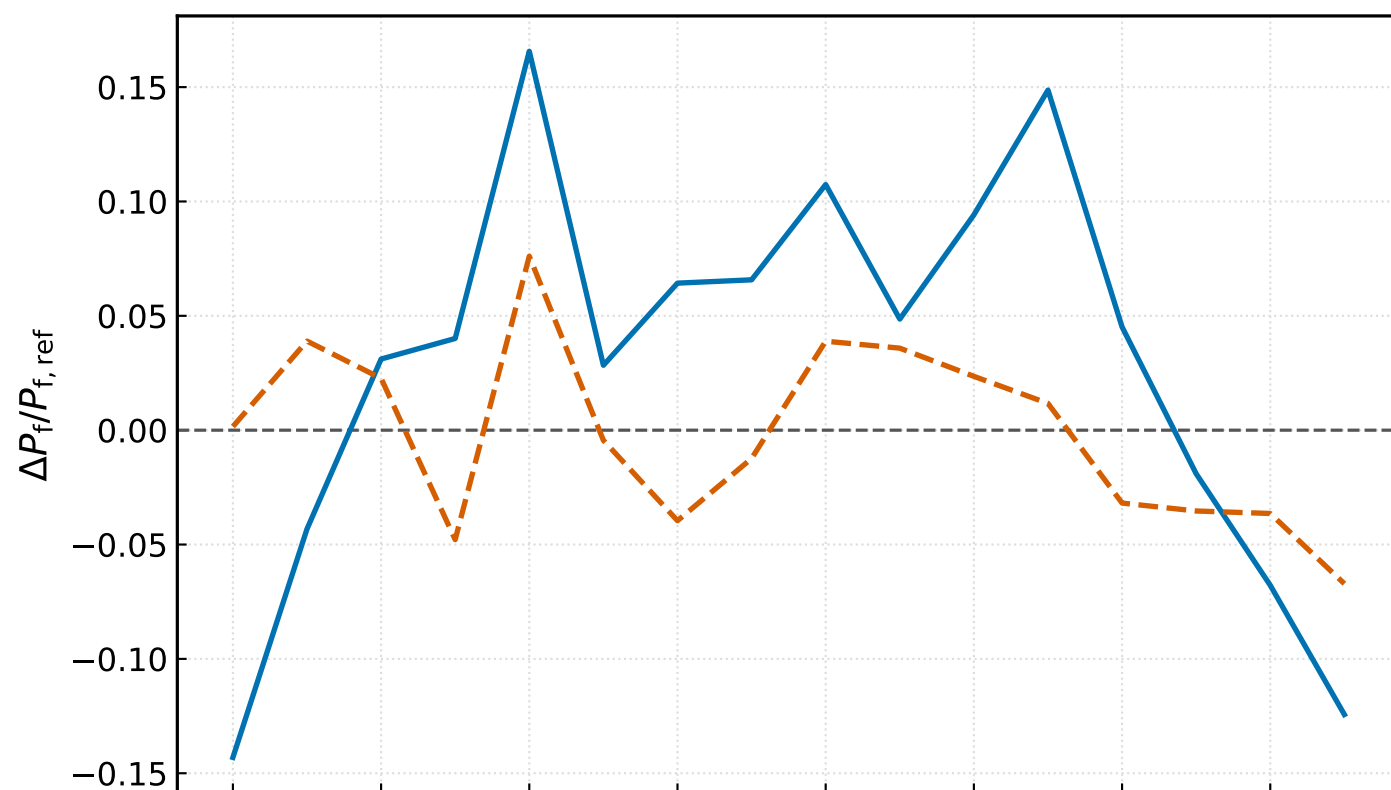
z = 4.2 : Box Size Relative Diff
