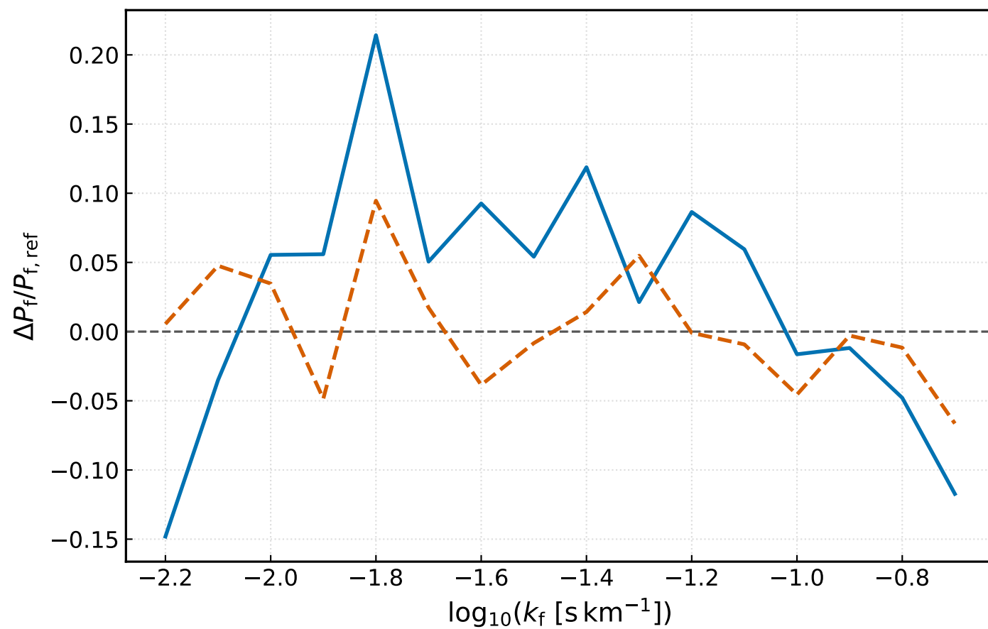
z = 4.2 : Box Size Relative Diff
