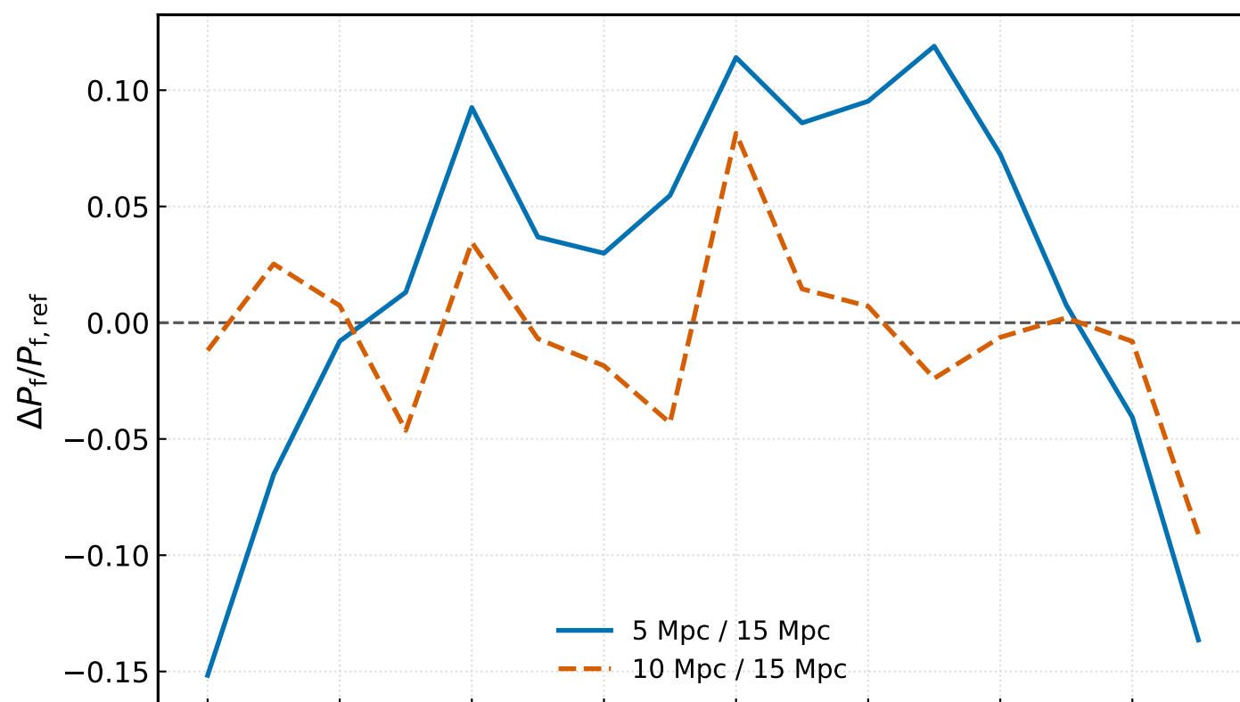
z = 4.6 : Box Size Relative Diff
