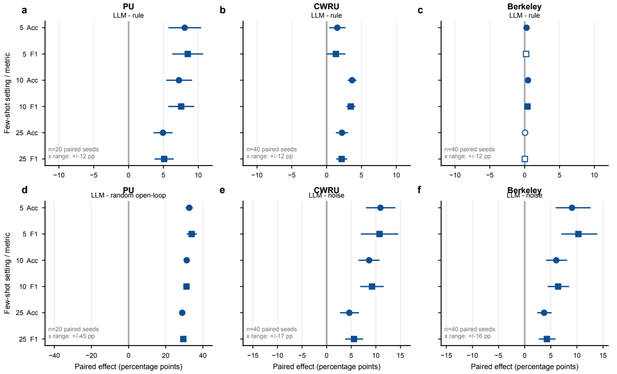
Figure 3: Paired downstream effects. Each marker is the paired mean LLM-comparator effect in percentage points over the registered seeds; lines are 95% percentile bootstrap intervals over paired seeds. (a–c) LLM minus rule on PU, CWRU within-load0, and Berkeley under one shared \pm 12 -point scale. (d–f) LLM minus random open-loop on PU and LLM minus noise augmentation on CWRU and Berkeley, with per-panel ranges printed. Circles are Accuracy and squares Macro-F1; filled markers pass the registered Holm correction and hollow markers do not. Seeds repeat few-shot subset selection and CNN initialization around one fixed pool per source.
