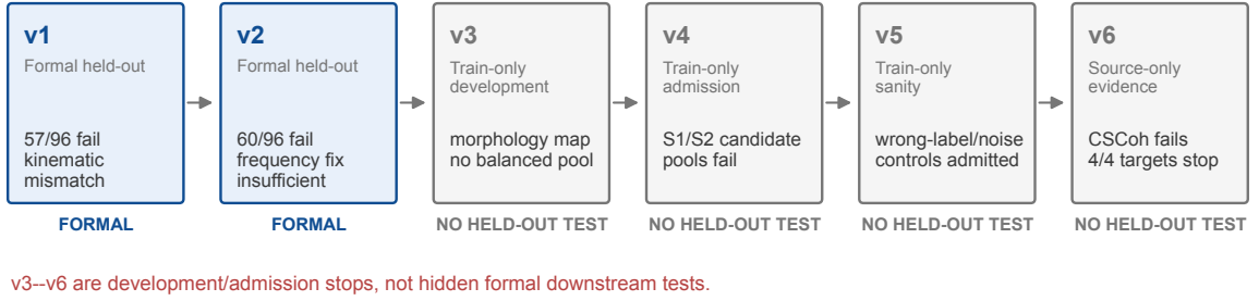
Figure 10: Complete PU LOCO failure chain. v1 and v2 are formal held-out evaluations; v3–v6 stop at train-only morphology, admission, sanity, or source-only evidence gates. The sequence prevents unsuccessful development stages from being reported as completed cross-condition tests.
