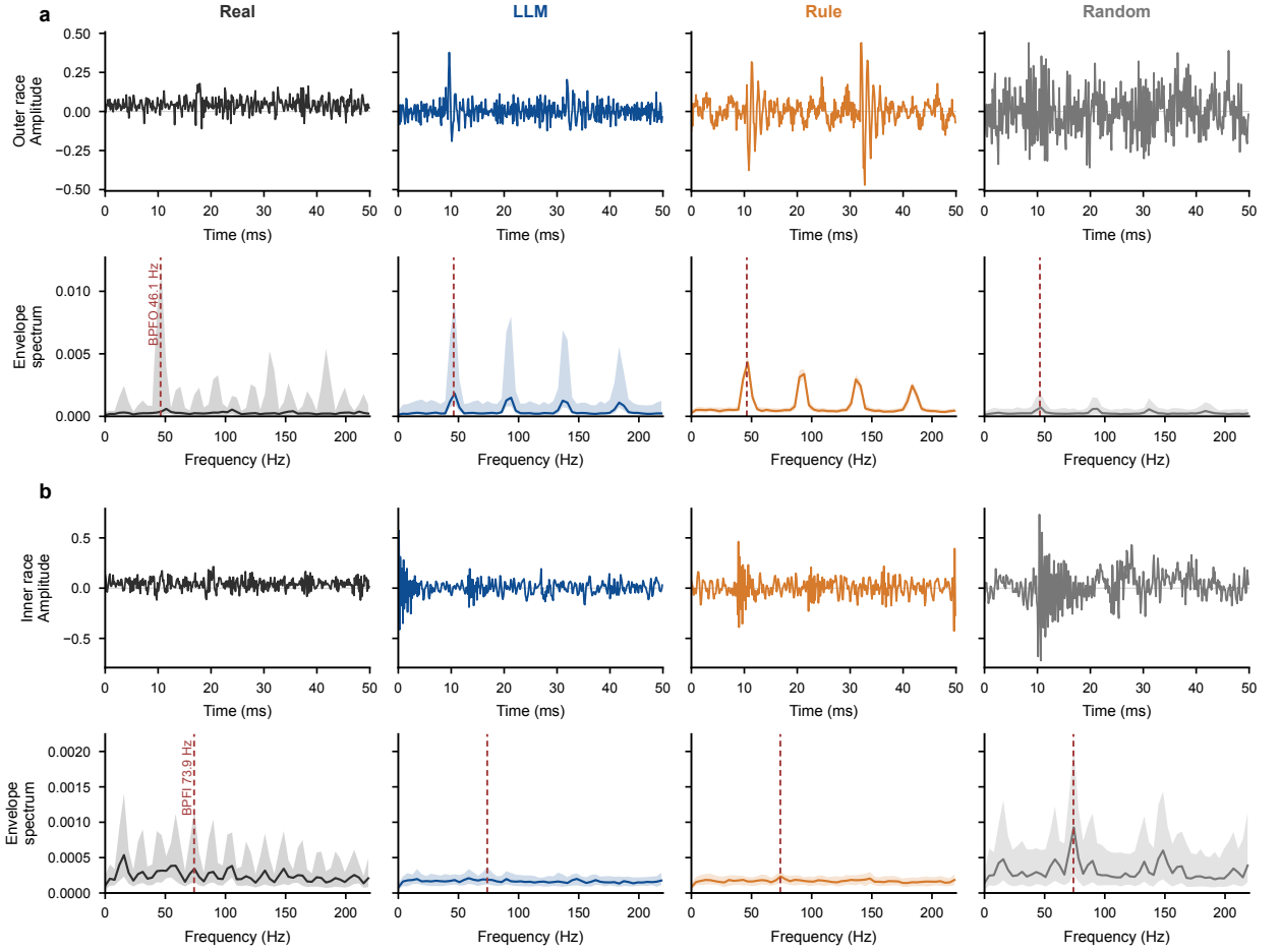
Figure 4: PU waveform and envelope-spectrum comparison for (a) outer-race and (b) inner-race classes; columns compare real training, LLM, rule, and random open-loop windows. Each waveform is the window nearest its source/class robust centre in a shared class-matched real-train-scaled feature space, with raw amplitude and shared class-specific y limits. Envelope spectra show the median and interquartile range over all windows of each source/class under the same fixed 500–2000 Hz demodulation band. Dashed markers denote the class-relevant kinematic frequency (BPFO 46.1 Hz; BPFI 73.9 Hz).
