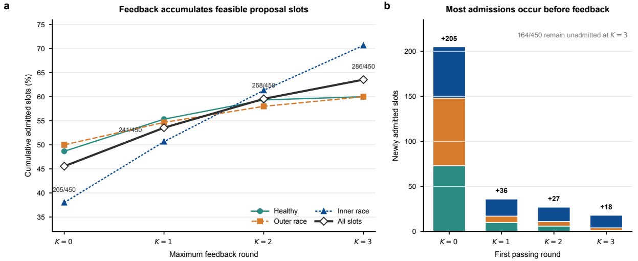
Figure 7: PU closed-loop admission across feedback rounds. (a) Cumulative percentage of proposal slots admitted by or before each round, shown for healthy, outer-race, and inner-race classes ( n = 150 slots each) and for all slots ( n = 450 ); labels give pooled cumulative counts. (b) Newly admitted slots assigned to their first passing round and stacked by class. A passing round is the earliest archived candidate with feasible=true ; the aggregate exactly reproduces the frozen 286 admitted slots, leaving 164 unadmitted at K = 3 . Counts describe one frozen pool-generation run and have no independent-pool sampling interval. Source data are provided with the figure artifacts.
