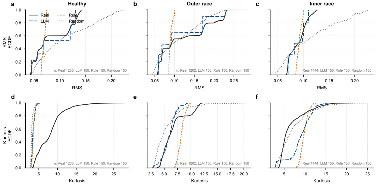
Figure 5: Class-conditional RMS (a–c) and kurtosis (d–f) empirical cumulative distributions for the real PU outer-training split and frozen synthetic pools. Real curves use every class-matched outer-training window (healthy/OR/IR: 1200/1202/1444), exactly the reference population used for the W1 diagnostics; synthetic curves use the fixed 150-window/class pools and are distinguished by both colour and line style. Admission narrows unsupported statistical excursions without forcing equality to a single reference value.
