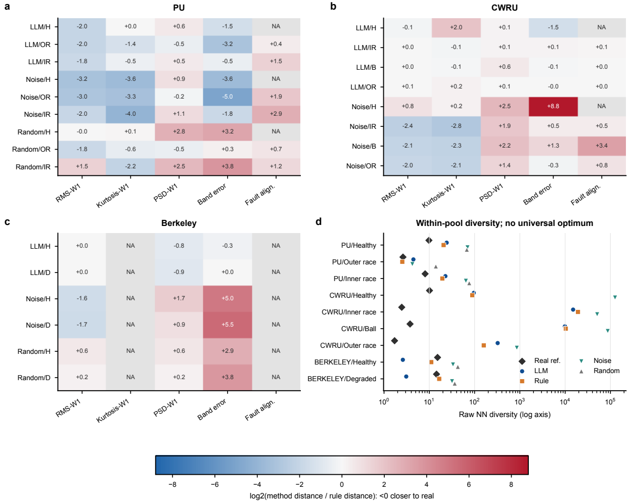
Figure 6: Class-specific physical diagnostics on (a) PU, (b) CWRU, and (c) Berkeley. Each matrix cell is \log_2 of the method-to-rule distance ratio for RMS-W1, kurtosis-W1, PSD-W1, relative band-energy error, and fault-frequency alignment; negative values favour the method and positive values favour rule, on one shared zero-centred scale. NA denotes a frozen metric that is undefined or unavailable, not an imputed value. (d) Within-pool nearest-neighbour diversity in raw units on a separate log axis; diversity has no universally optimal direction and does not share the fidelity colour scale.
