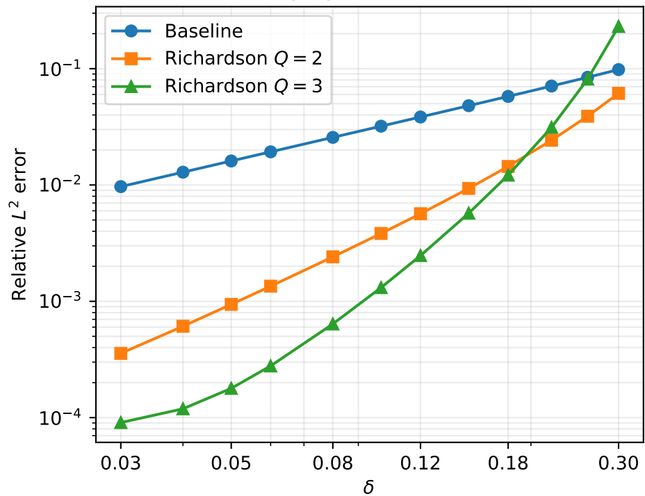
Symplectic Euler
