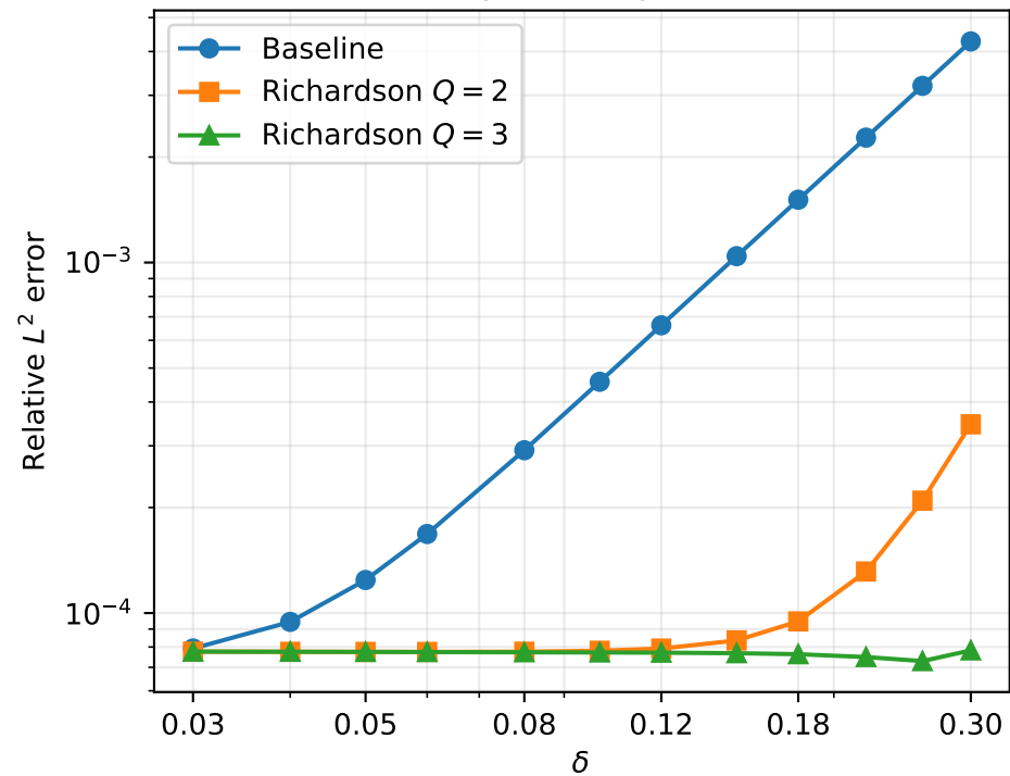
Implicit Midpoint
