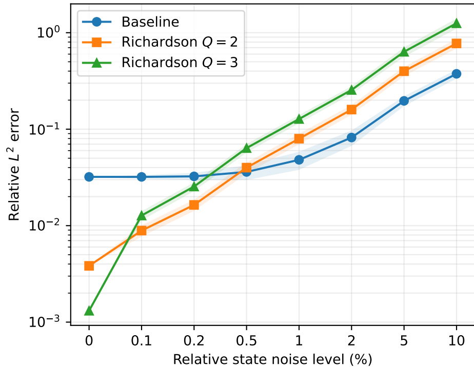
Symplectic Euler
