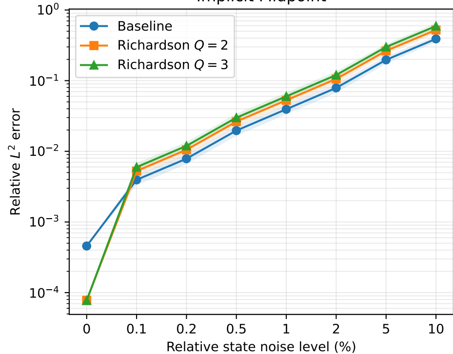
Implicit Midpoint
