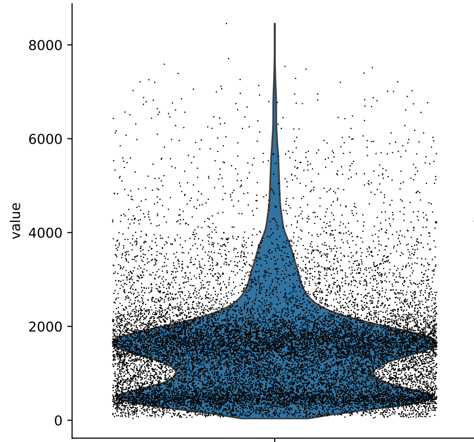
n_genes_by_counts
