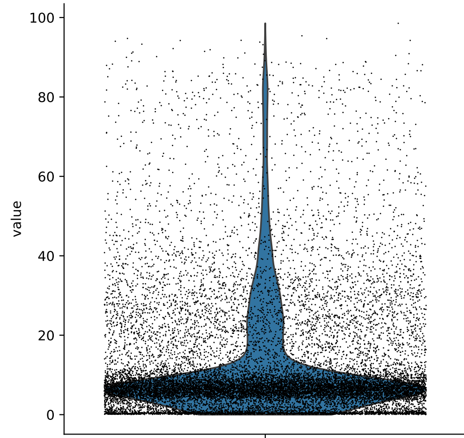
pct_counts_mt
