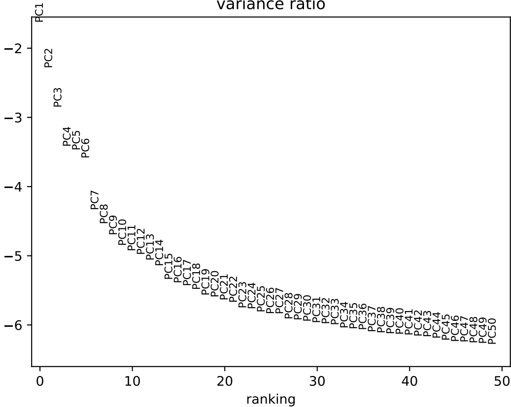
variance ratio
