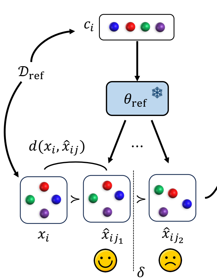
(b) Preference Dataset Construction
