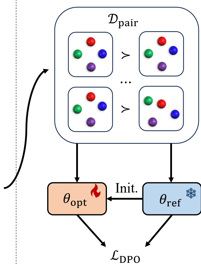
(c) Direct Preference Optimization
