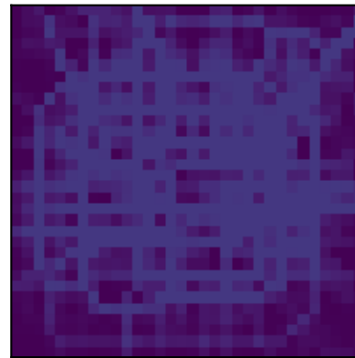
Inverse order
