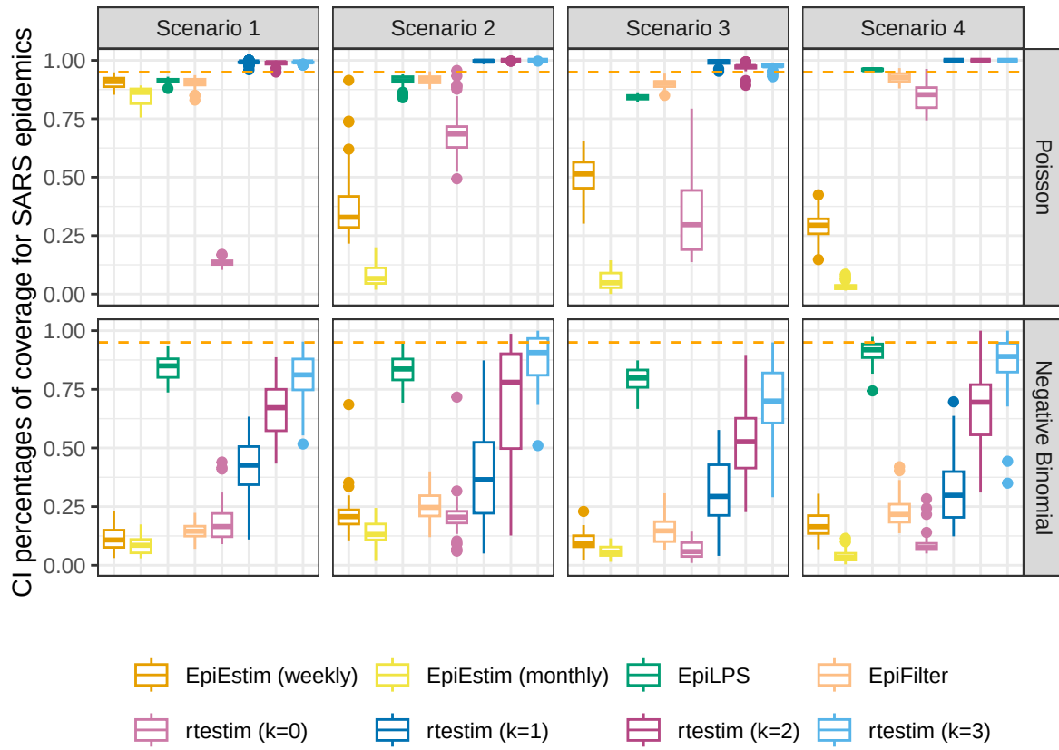
Fig A.6.8: Percent coverage of CIs over all timesteps for 50 synthetic SARS epidemics. The orange dashed line represents 95% percentage of coverage across all timesteps.
