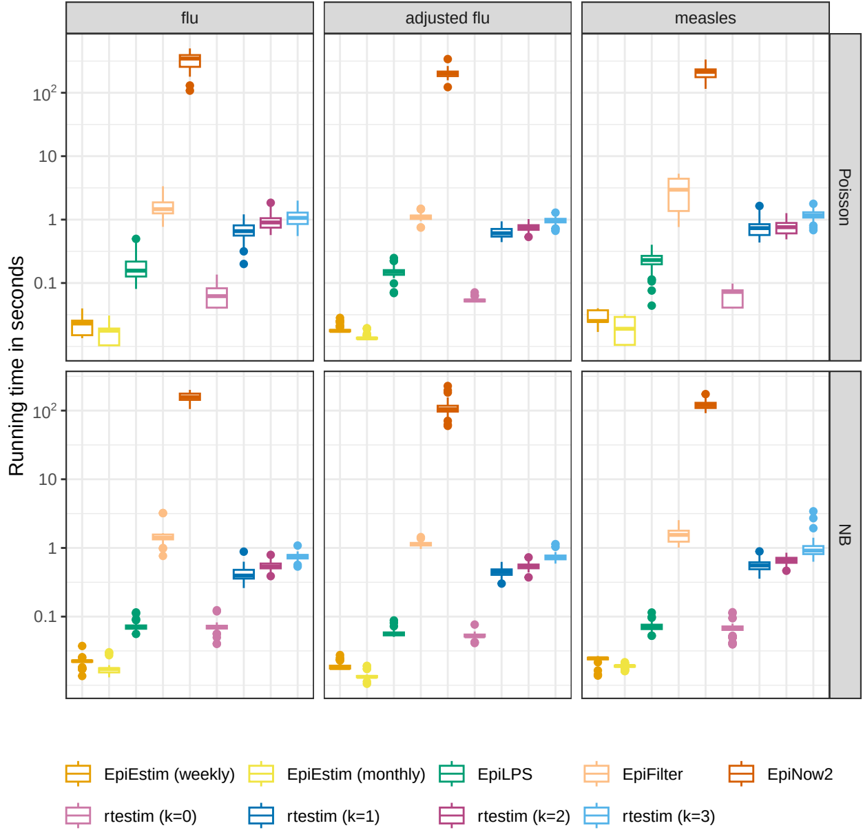
Fig A.5.5: Time comparisons of methods for short (flu) epidemics for piecewise linear R_t (Scenario 3) for different pairs of SI parameters (flu, adjusted flu, and measles) and incidence distributions in different panels. Y-axes are on a logarithmic scale.
