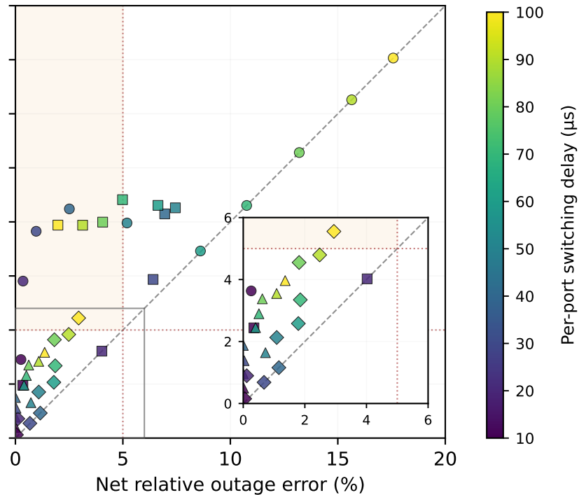
Fully space-time separable
