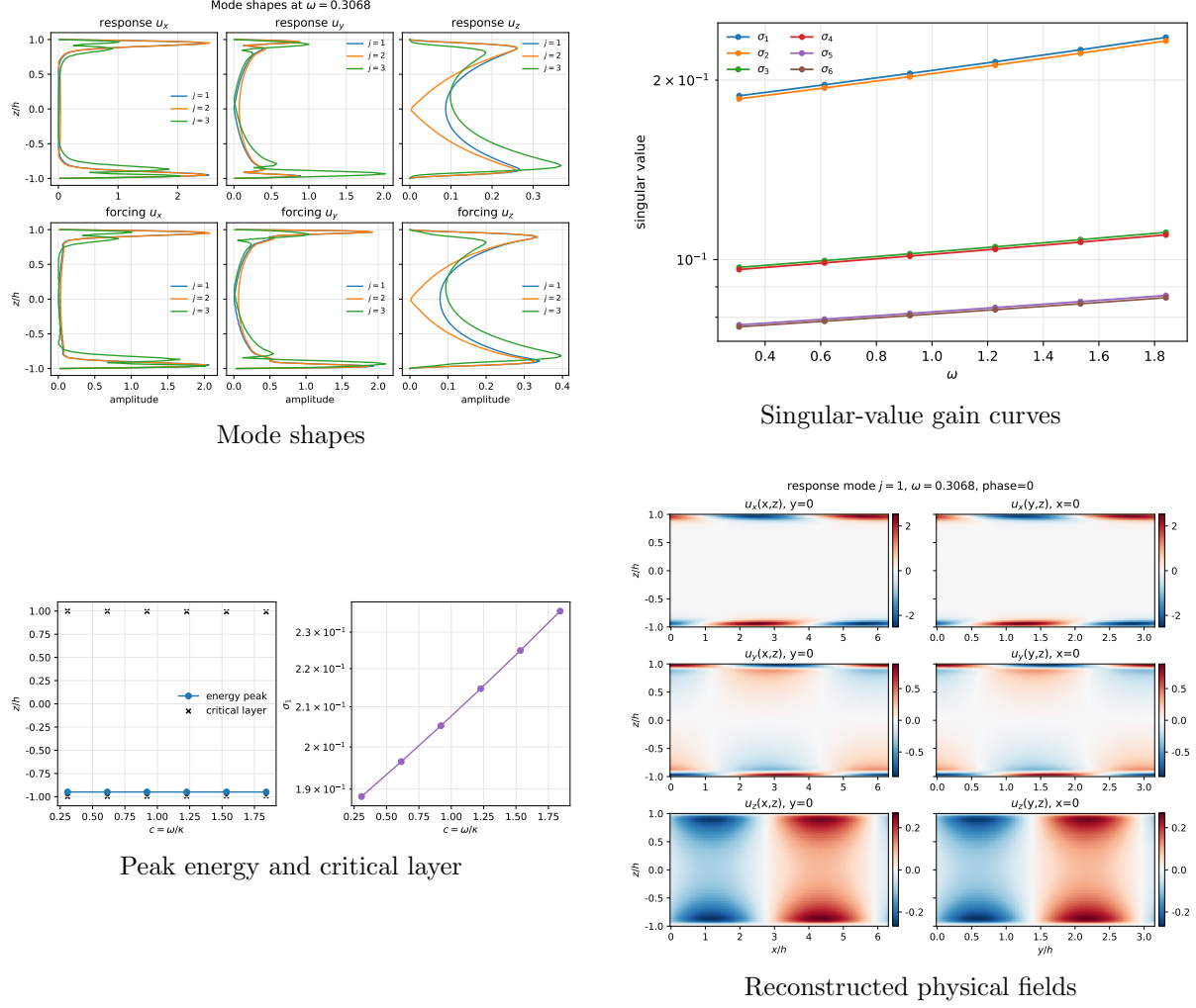
Figure 12: Dense temporal-CSD selected-mode resolvent figures for mode (1, 1), corresponding to (\kappa, \lambda) = (1, 2) .
