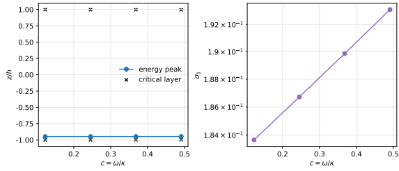
Peak energy and critical layer
