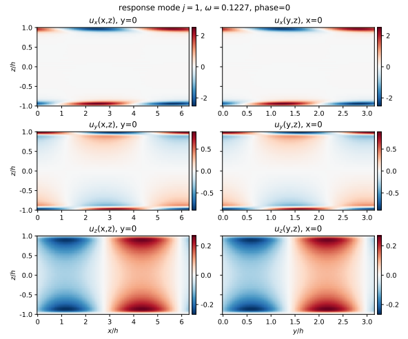
Reconstructed physical fields
