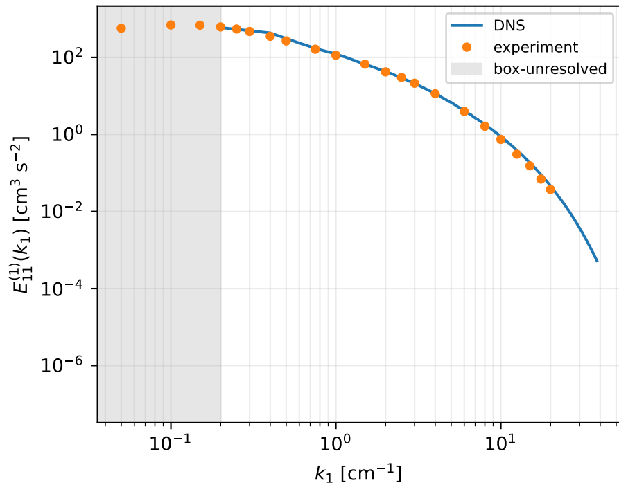
tU_0/M = 42
