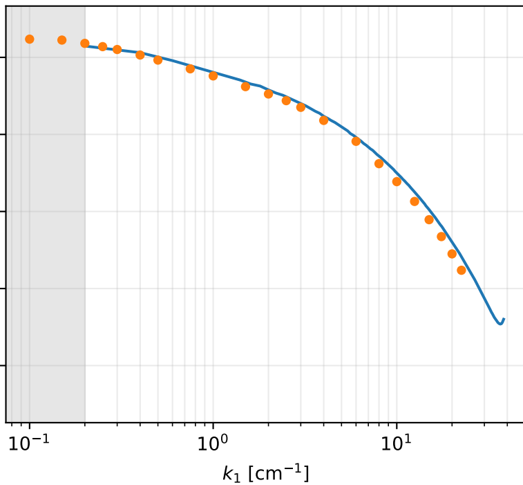
tU_0/M = 98
