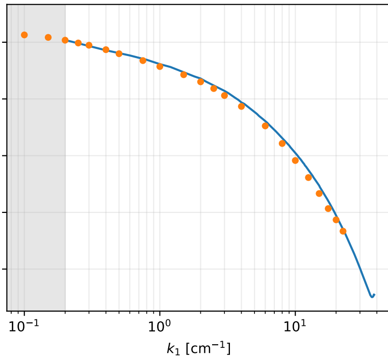
tU_0/M = 171
