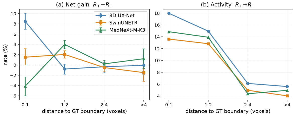
Figure 5: Boundary-resolved decoder benefit versus physical distance to ground-truth boundary ( d_{GT} ) across backbones: (a) net gain R_+ - R_- , and (b) activity R_+ + R_- .
