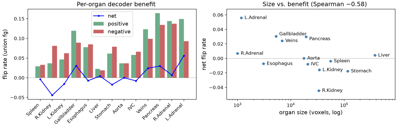
(b) SwinUNETR Organ-Level Flips
