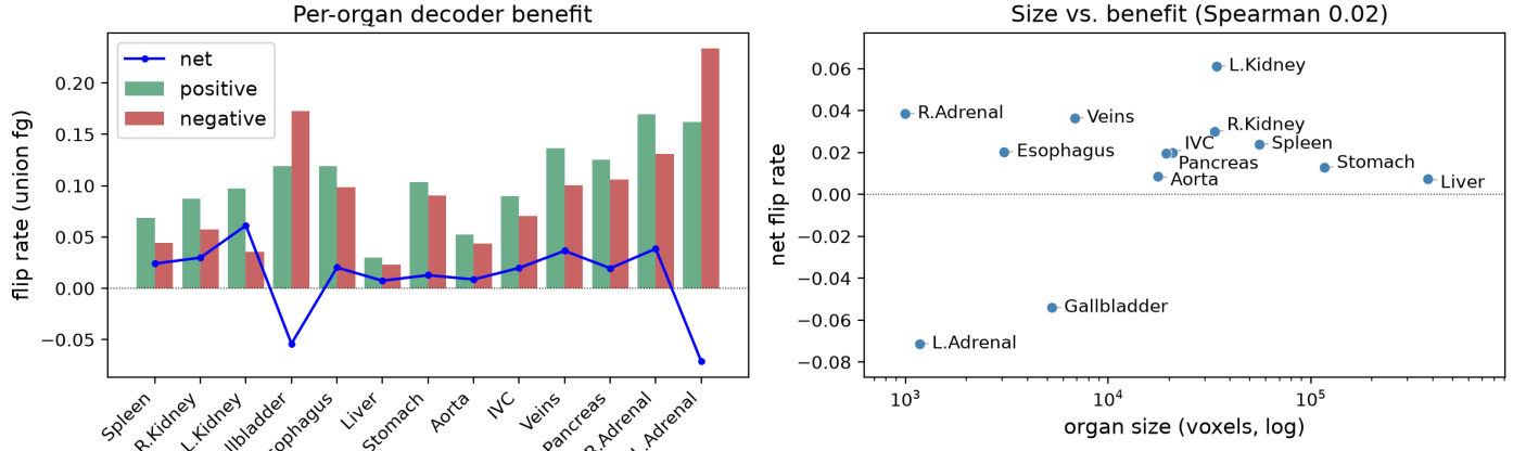
(a) 3D UX-Net Organ-Level Flips
