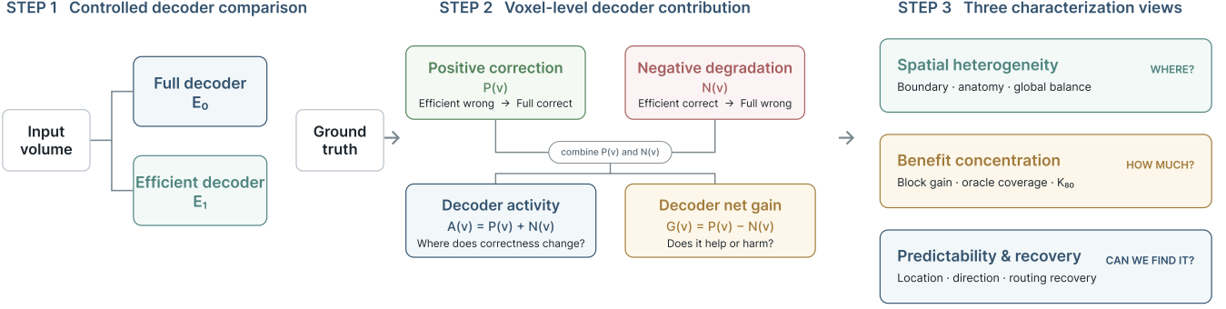
Figure 1: Overview of the decoder-computation characterization framework. Step 1 (Controlled Decoder Comparisons): Full and efficient decoder pairs are evaluated under two complementary regimes (independently trained end-to-end pairs for cross-architecture consistency, and frozen shared-encoder factorials for decoder-isolated causal attribution). Step 2 (Voxel Activity and Net Gain): Voxel-level corrections and degradations establish the fundamental dichotomy between Decoder Activity (where the decoder acts) and Net Gain (where it helps). Step 3 (Three Characterization Axes): Probes spatial heterogeneity, benefit concentration, and predictability. Step 4 (Design Implications): Translates empirical insights into evidence-backed directions for adaptive decoder design.
