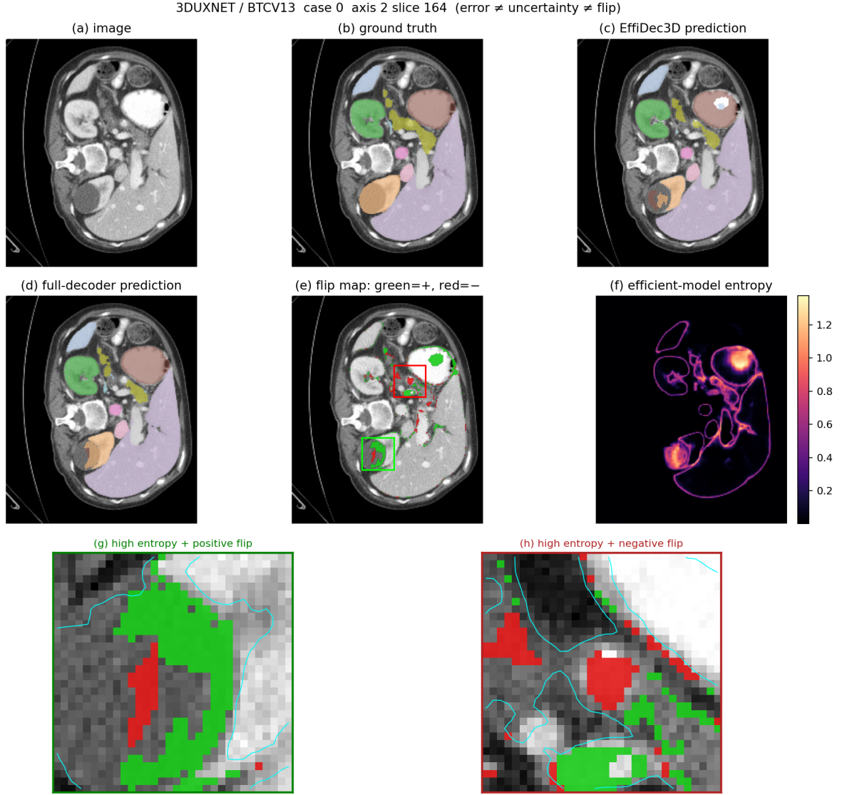
Figure 2: Qualitative illustration of decoder activity and directional gain (3D UX-Net on BTCV CT multi-organ dataset). While the full decoder corrects certain errors of the efficient baseline (positive flips), it also alters previously correct predictions (negative flips) near high-entropy organ boundaries, demonstrating non-uniform spatial contribution (see Supplementary Figures S1 and S2 for SwinUNETR and MedNeXt-M-K3).
