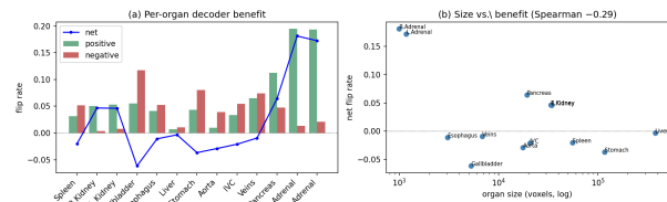
Figure 2. H2, per-organ net flip for the matched pair (seed 1): positive, negative, and net rates on each organ’s union (GT, Full, Effi) foreground, and net flip vs. organ size. The decoder’s net benefit is uneven across anatomy and rises as structures shrink.
