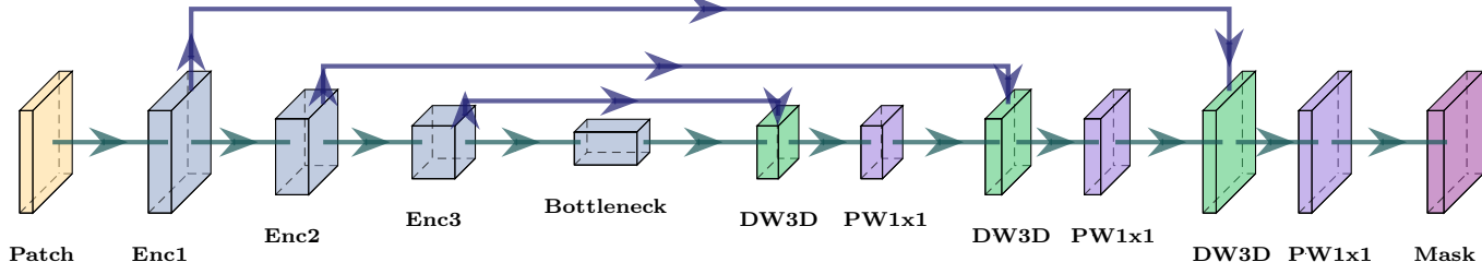
Separable ( E'_1 ): C_{384} , All Stages, DW 3D Conv + PW 1x1x1 Conv (37.3M Params, 174.0 GMac)
