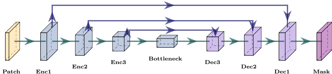
EffiDec3D ( E_1 ): C_{48} (-87.5%), Stage 1 Omitted (3.2M Params, 49.5 GMac)
