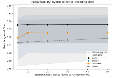
(c) MedNeXt-M-K3 Macro Recovery
