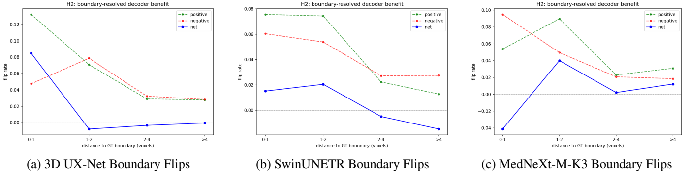
Figure 4: Spatial ground-truth boundary concentration of prediction flips across the three evaluated backbones.
