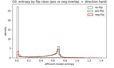
(c) MedNeXt-M-K3 Flip Entropy Density
