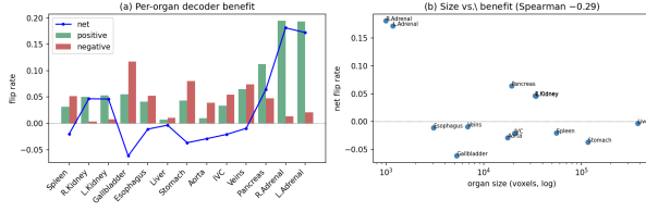
Figure 1. H2, per-organ net flip for the matched pair (seed 1): positive, negative, and net rates within each organ’s GT voxels, and net flip vs. organ size. The decoder’s net benefit is uneven across anatomy and rises as structures shrink.
