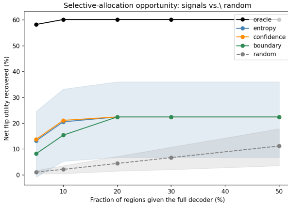
Figure 2. C1/P2: net benefit recovered vs. the fraction of 16^3 blocks selected. The true-net oracle (black; C1) upper-bounds concentration, while deployable signals (entropy, confidence, boundary) and a matched-random selector (P2) show whether that opportunity is recoverable at test time. Shaded bands are subject 95% CIs.
