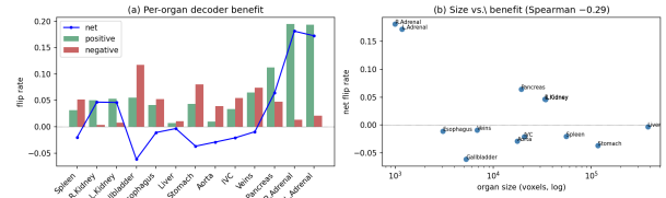
Figure 2. H2, per-organ net flip for the matched pair (seed 1): positive, negative, and net rates on each organ’s union(GT, Full, Effi) foreground, and net flip vs. organ size. The decoder’s net benefit is heterogeneous across anatomy—some structures gain, others lose—with no robust size trend.
