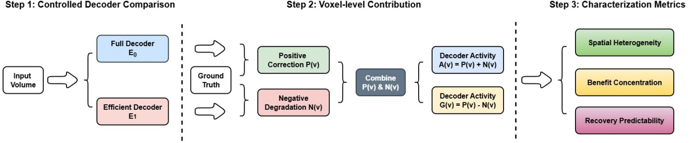
Figure 1: Overview of the decoder computation characterization framework across Step 1 (Controlled Interventions), Step 2 (Voxel Correctness Activity A_{\text{corr}}(v) and Net Gain G(v) ), and Step 3 (Three Characterization Axes).
