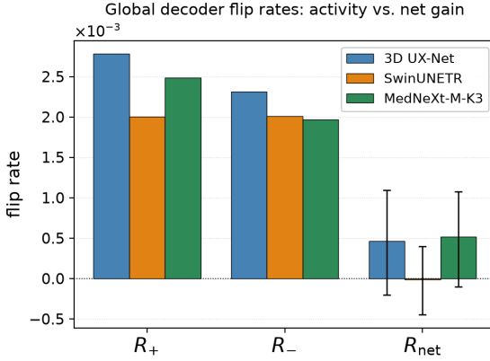
Figure 3: Global flip rates for all three backbones under Full ( E_0 ) vs. Efficient ( E_1 ) decoders, grouped by quantity. Positive corrections R_+ and negative degradations R_- are large and comparable (bidirectional activity), whereas the net gain R_{net} is near zero with a subject-bootstrap 95% CI that includes zero for every backbone.
