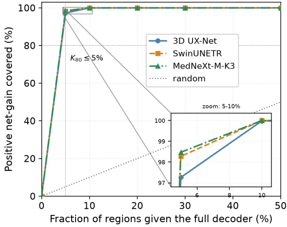
Figure 6: Oracle positive-gain concentration for the three backbones (inset: zoom on the 5–10% separation). All satisfy K_{80} \leq 5\% ; the gray dashed line is the random baseline.
