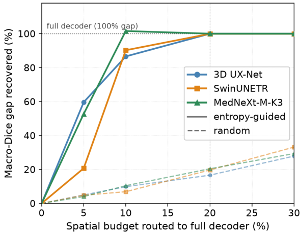
Figure 8: Macro-Dice gap recovery under output hybridization for the three backbones, as a percentage of the full-minus-efficient Dice gap. Solid = entropy-guided routing, dashed = random baseline. Entropy-guided routing recovers the full gap by a 20% budget for all three backbones, versus \sim 20\% for random selection.
