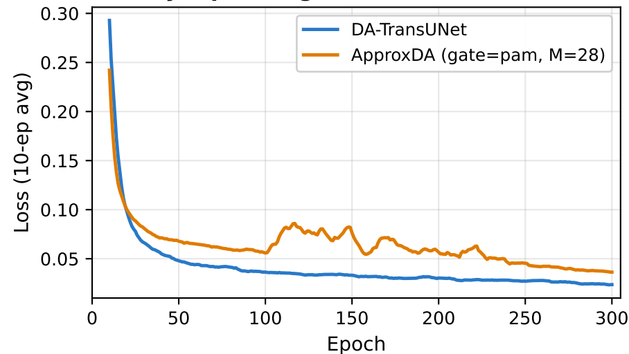
Synapse (High-GCS) — Train Loss
