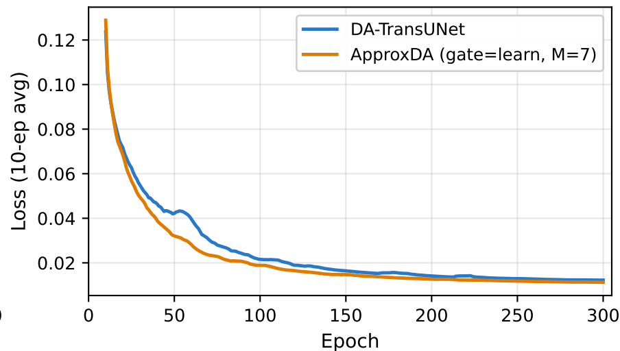
Kvasir-SEG (Low-GCS) — Train Loss
