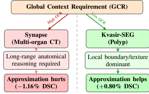
Fig. 6. GCR governs approximation effectiveness. A task’s Global Context Requirement determines whether approximation is beneficial or harmful: the same ApproxDA configuration yields opposite effects on high-GCR and low-GCR benchmarks.
