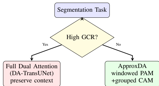
Fig. 7. Practical design guideline derived from GCR analysis. Tasks requiring cross-organ anatomical reasoning (high GCR) should retain full dual attention. Local-structure tasks (low GCR) can safely use ApproxDA, reducing per-GPU VRAM by 44% with no accuracy penalty.
