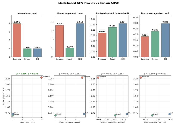
Fig. 9. Mask-based proxy metrics vs. known \Delta DSC. n_{\text{classes}} (leftmost) shows the strongest Spearman correlation ( \rho = +0.87 ). Spatial metrics (centroid spread, bbox coverage) show wrong-direction correlations, consistent with the SC1/SC3 elimination.
