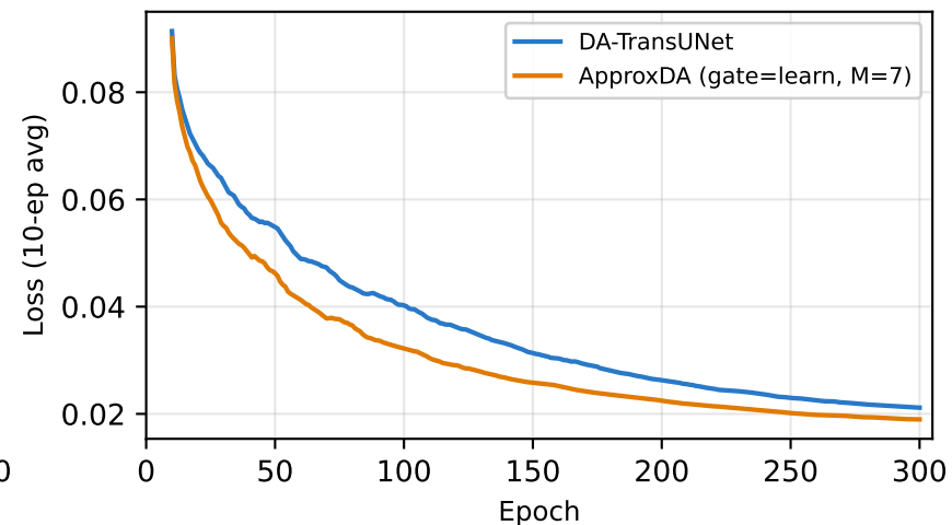
ISIC 2018 (low CS) — Train Loss
