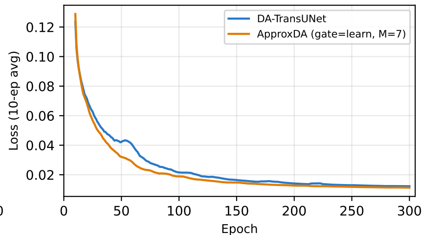
Kvasir-SEG (low CS) — Train Loss
