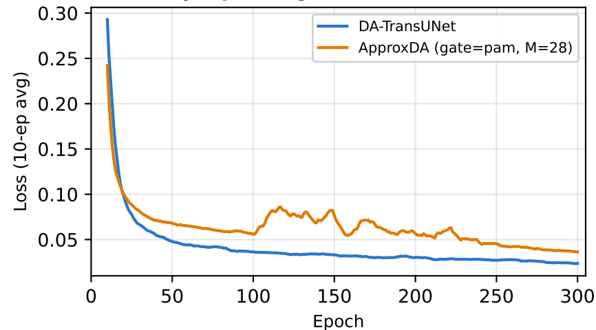
Synapse (high CS) — Train Loss
