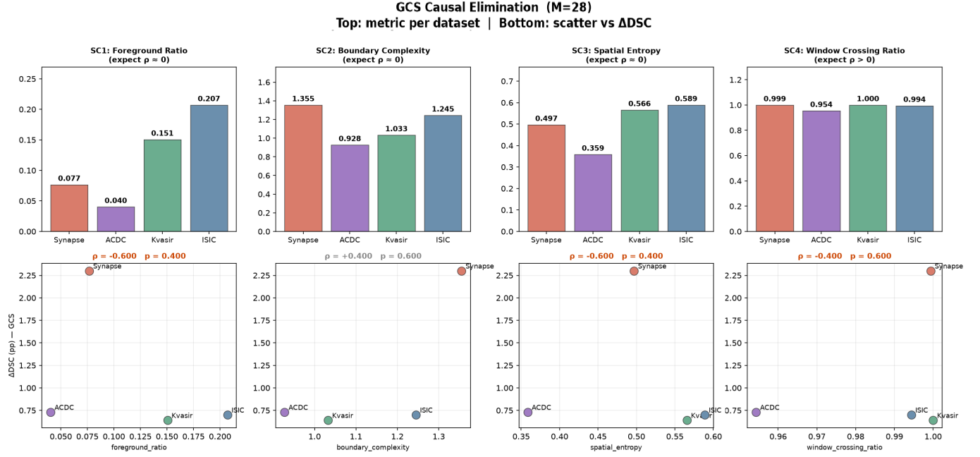
Fig. 8. Causal elimination results ( M=28 , 200 masks/dataset, four datasets including ACDC). Top row: per-dataset metric values. Bottom row: scatter vs. known \Delta DSC (GCS). SC1 and SC3 show wrong-direction correlations; SC4 saturates across all datasets; SC2’s apparent confound ( \rho = +1.00 on three datasets) collapses to \rho = +0.40 once ACDC is included. All four alternative explanations are eliminated; SC5 ( \rho = +0.95 ) is the only metric that cleanly predicts GCS.
