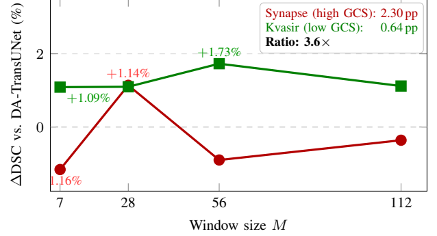
Fig. 4. \Delta DSC vs. window size M (gate=pam, r=32 ) for Synapse (red, high GCS) and Kvasir-SEG (green, low GCS). Annotation box: DSC span and 3.6\times ratio.
