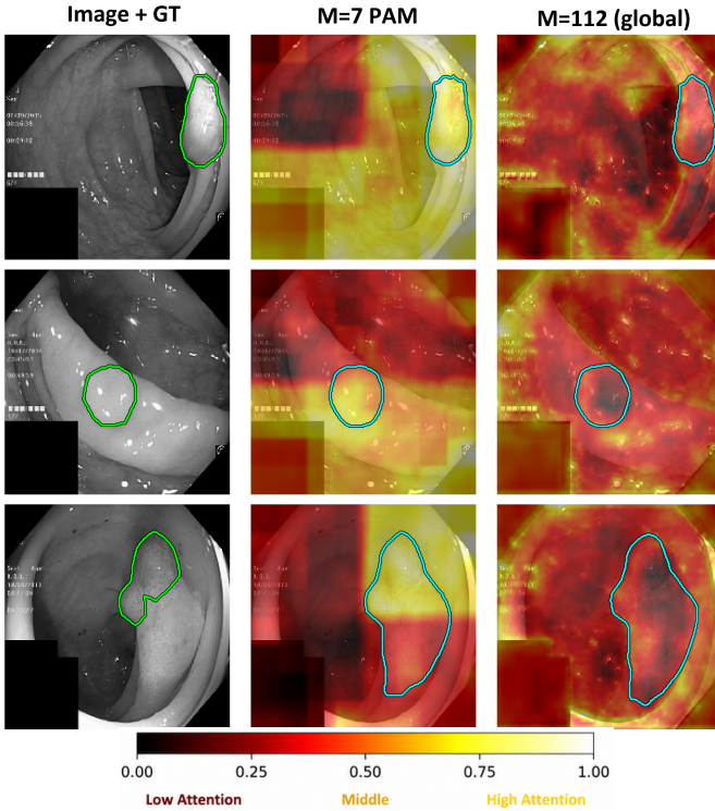
Fig. 5. PAM contribution maps ( \|output - input\|_2 , per-panel normalised; colorbar below) on three Kvasir-SEG polyp images. Each row: input with GT contour (left), windowed PAM ( M=7 ; center), global PAM ( M=112 ; right). Brighter color indicates larger PAM contribution at that location; panels are independently normalised so magnitudes are not comparable across panels.
