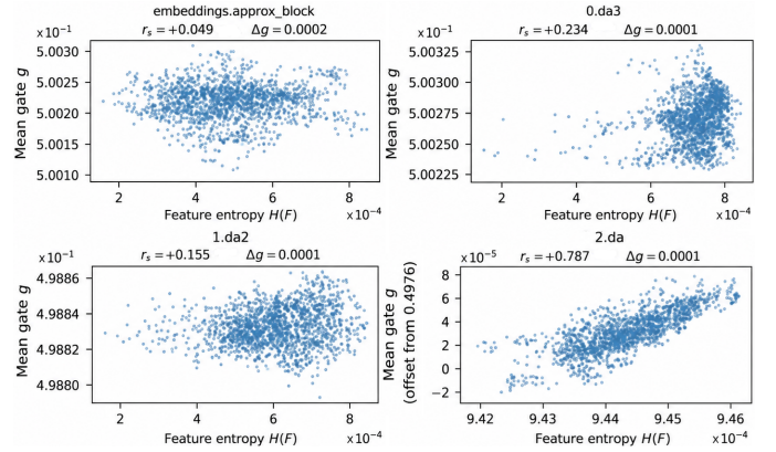
Fig. 6. Gate value g vs. feature entropy H(F) at all four skip locations ( M=7 , \text{gate}=\text{learn} ): bottleneck, 28^2 , 56^2 , 112^2 . All cluster at g \approx 0.5 ( \Delta g \leq 0.0002 ), confirming gate collapse.
