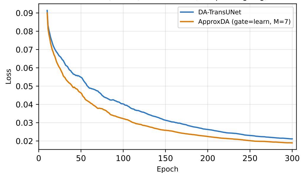
ISIC 2018 (low CS) — Train Loss (10-ep rolling avg)
