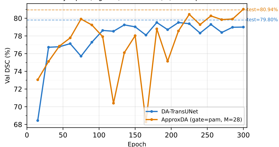
Kvasir-SEG (low CS) — Val DSC (%) over epochs
