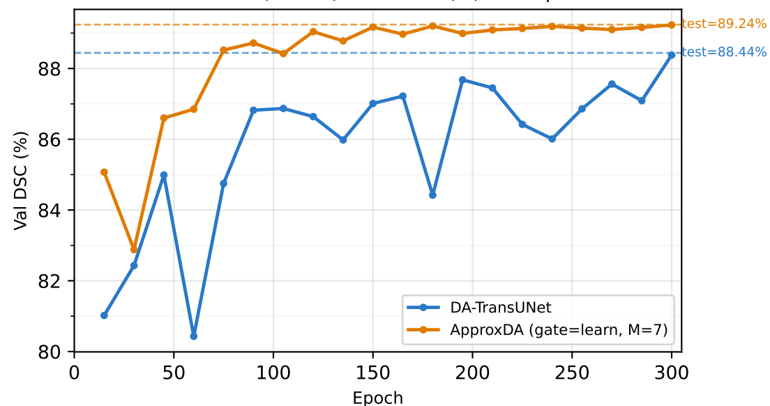
ISIC 2018 (low CS) — Val DSC (%) over epochs
