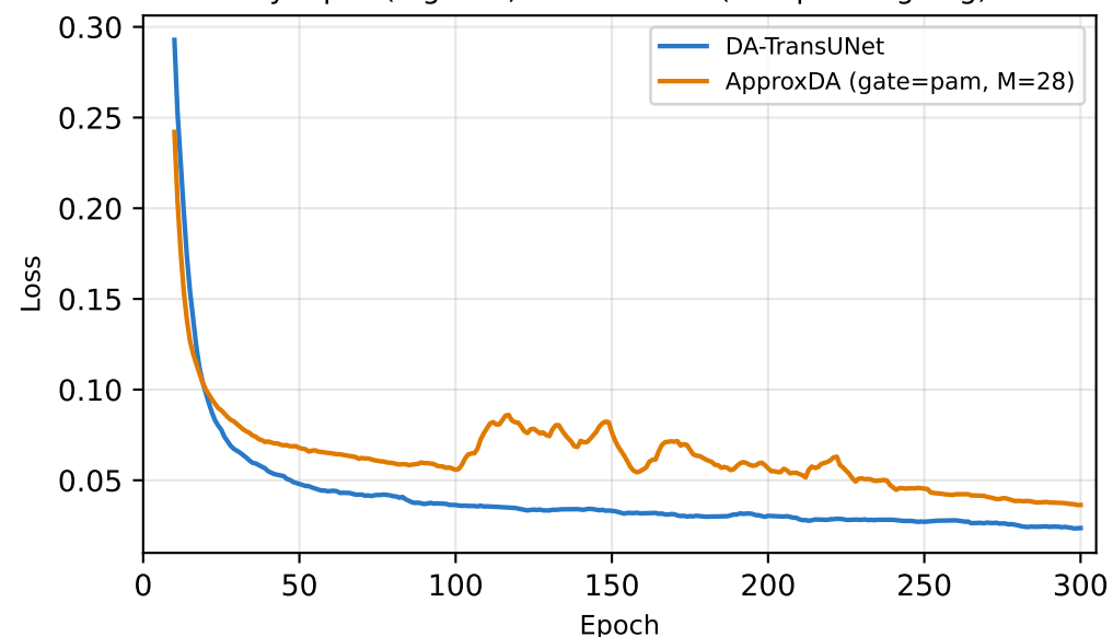
Kvasir-SEG (low CS) — Train Loss (10-ep rolling avg)
