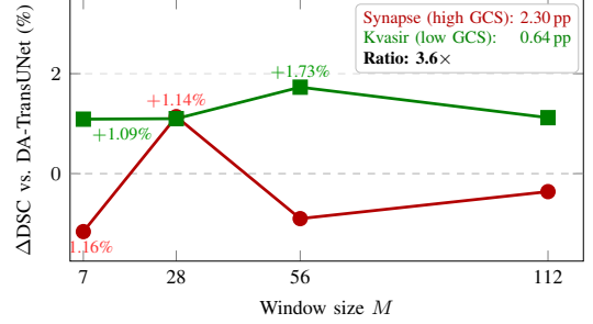
Fig. 4. Per-window gain of ApproxDA-TransUNet over DA-TransUNet ( \Delta DSC, gate=pam, r=32 ). The Synapse curve (red) spans 2.30 pp and crosses zero: wrong window choices actively hurt on this empirically high-GCS task. The Kvasir-SEG curve (green) spans only 0.64 pp and stays positive throughout: any reasonable window helps on this empirically low-GCS task. The 3.6 \times span ratio (annotation box) directly operationalizes empirical GCS.
