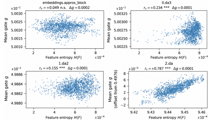
Fig. 6. Gate value vs. per-block feature entropy H(F) ( M=7 , gate=learn). Panels (TL→BR): embeddings.approx_block (bottleneck), 0.da3, 1.da2, 2.da (skip connections at 28^2 , 56^2 , 112^2 ). All four locations collapse to g\approx 0.5 with \Delta g\leq 0.0002 , confirming uniform gate collapse across scales.
