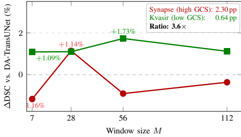
Fig. 4. Per-window gain of ApproxDA-TransUNet over DA-TransUNet ( \Delta DSC, gate=pam, r=32 ). The Synapse curve (red) spans 2.30 pp and crosses zero: wrong window choices actively hurt on this empirically high-GCS task. The Kvasir-SEG curve (green) spans only 0.64 pp and stays positive throughout: any reasonable window helps on this empirically low-GCS task. The 3.6\times span ratio (annotation box) directly operationalizes empirical GCS.
